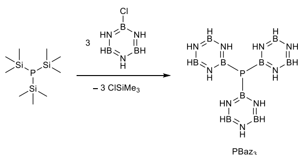
Scheme 1. Synthesis of tris(2-borazinyl)phosphine ( \text{PBaz}_3 ).
