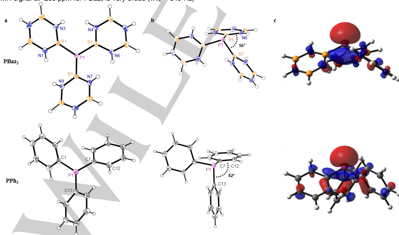
Figure 3. Molecular structures of \text{PBaz}_3 and \text{PPh}_3 . [42] Two views of the structures are given: (a) along the C_3 axis and (b) perpendicular to the C_3 axis, to facilitate the comparison. (c) Plots of the HOMOs of \text{PBaz}_3 and \text{PPh}_3 (isovalues 0.05). Selected bond lengths (Å) and angles: P1–B1 1.923(2), P1–B4 1.9230(19), P1–B7 1.9255(18), B1–P1–B4 106.34(8), B4–P1–B7 107.78(8), B1–P1–B7 107.44(8), B1–P1–B7–N9 52.94(11), B7–P1–B4–N6 55.98(10), B4–P1–B1–N3 57.74(10).
