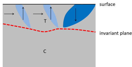
Figure 3. The sketch is a side view of the sample polarization state, for temperature above T_C . The surface is represented by a dark line and the invariant plane by a red dashed line. The bulk is in the cubic (C) phase, while the surface remains in the tetragonal (T) phase. The polarization directions are represented by dark arrows.
