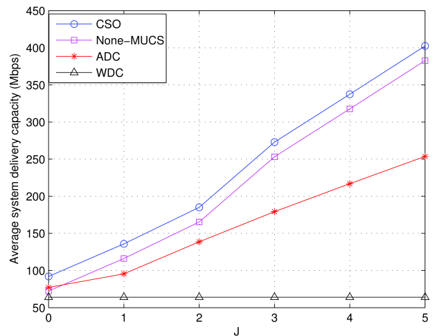
FIGURE 9. Capacity performance versus number of FBSSs J .
