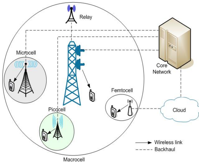
Figure 5. Network Architecture of a 5G HetNet.
