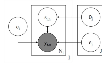
Figure 3: Plate diagram for the MACE model.
