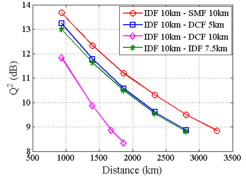
Fig. 7. Q^2 vs transmission distance for different dual-stage DRA schemes.
