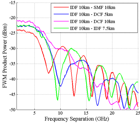
Fig. 4. Experimental product power as a function of the frequency separation between two CW lasers (3dBm each).
