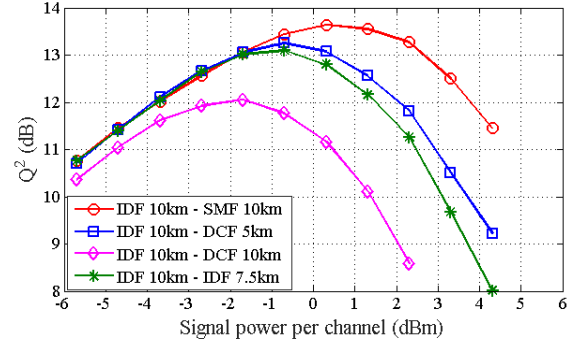
Fig. 6. Q^2 vs signal power per channel for different dual-stage DRA schemes for 10 spans of 93.4km transmission length for 194THz channel.
