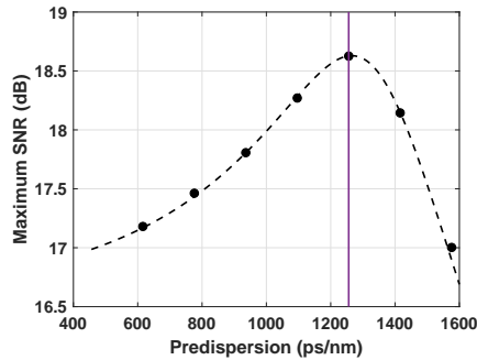
Fig. 3: The Maximum signal to noise ratio (SNR) of the central channel of 17 WDM channels as a function of the pre-dispersion for theory (dashed line) and simulation (markers). The optimum pre-dispersion (vertical line).
