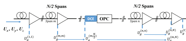
Fig. 1: Block diagram for mid-link OPC system with pre-dispersion. DCE: Dispersion Compensating Element, U_g^{(1,1)} : the FWM field from the first span and N : Number of spans
