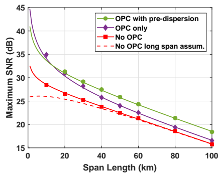
Fig. 4: The Maximum signal to noise ratio (SNR) of the central channel of 17 WDM channels as a function of the span length in three cases: Without OPC (red), with OPC only (purple) and with OPC and pre-dispersion (green) for theory (lines) (Eq.(11) (solid), Eq.(21) in [12] (dashed)) and simulation (markers).
