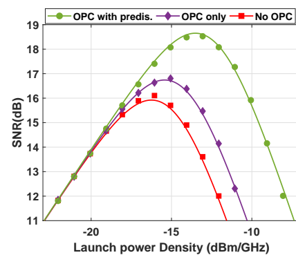
Fig. 2: The signal to noise ratio (SNR) of the central channel of 17 WDM channels as a function of the total launched power density in three cases: Without OPC (red squares), with OPC only (purple diamonds) and with OPC and pre-dispersion (green circles) for theory (lines) and simulation (markers).
