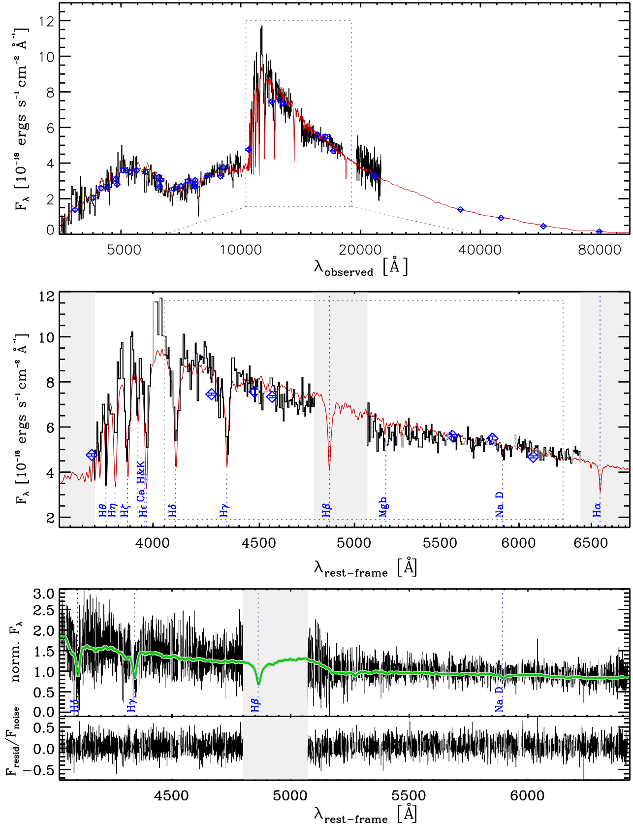
FIG. 1.— X-Shooter spectrum of NMBS-C7447 and the best-fit stellar population model (red line). Top panel: broad and medium-band data (blue diamonds) in combination with low-resolution spectrum ( 10 \text{ \AA} per bin). The entire wavelength range from UV ( 0.35 \mu\text{m} ) to NIR ( 2.3 \mu\text{m} ) is covered in 2 hr integration time with unprecedented quality. The galaxy is best fit with a young stellar population (0.40 Gyr, \tau = 0.03 \text{ Gyr} ) with little star formation ( 0.002 M_{\odot} \text{ yr}^{-1} ), and a stellar mass of M_{\star} \sim 1.5 \times 10^{11} M_{\odot} . Middle panel: Zoom in on the rest-frame optical part of the spectrum. Grey areas indicate regions of strong skylines or atmospheric absorption. Most prominent stellar absorption features are indicated with blue dashed line. Bottom two panels: High resolution spectrum ( 0.5 \text{ \AA} bin) of the observed features used to determine the stellar velocity dispersion. Green line is the best fit for the velocity dispersion with 4020 \text{ \AA} < \lambda_{\text{rest-frame}} < 6400 \text{ \AA} using the pPFX code (Cappellari & Emsellem 2004). The resulting stellar velocity dispersion is \sigma_{\star} = 294 \pm 51 \text{ km s}^{-1} . The residual from the best fit divided by the noise is shown in the bottom panel.
