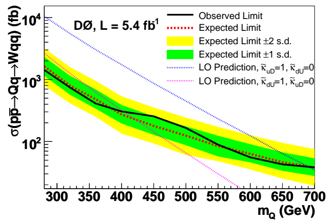
FIG. 3: Excluded production cross section for a vector-like quark Q decaying to Wq as a function of m_Q , compared to LO predictions of vector-like quark production with different \tilde{\kappa}_{qQ} .
