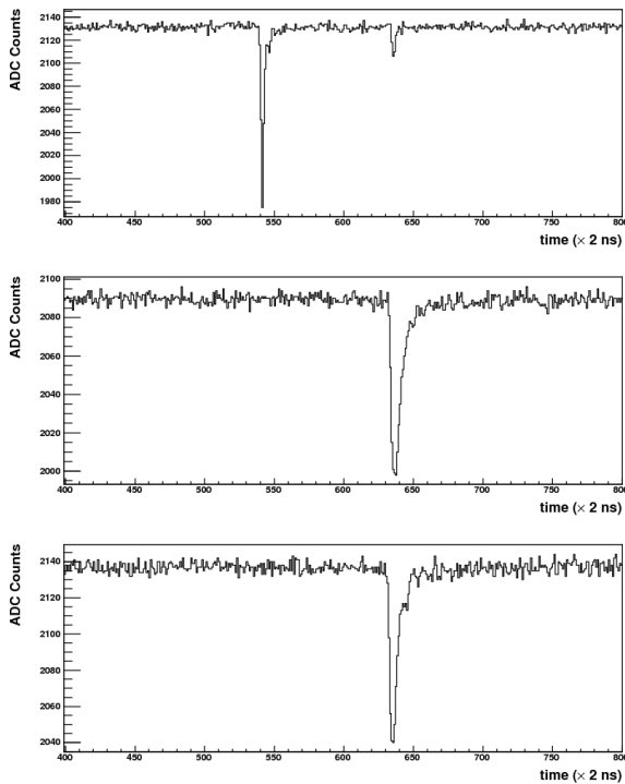
Figure 4. The signal of a train of bunches for the Cherenkov rod (top plot) and the two veto counters (middle and bottom plots). Two particles in two different bunches can be observed: the first one passes through the rod while the second one passes through both veto counters (and leaves also a small signal in the rod when it hits the PMT glass producing a small amount of Cherenkov in it).
