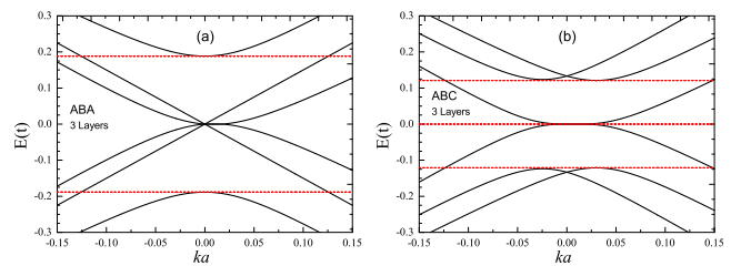
FIG. 9. (Color online) Band structure of ABA- and ABC-stacked trilayer graphene. Left panel: the red dashed lines indicate the position of the jump in DOS of ABA-stacked trilayer graphene at |E| \approx 0.19t . Right panel: the red dashed lines indicate position of the peaks in DOS of ABC-stacked trilayer graphene at E = 0 and |E| \approx 0.12t .
