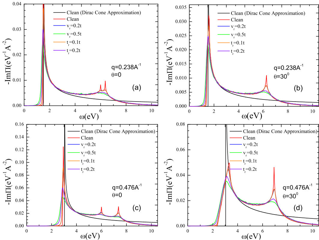
FIG. 5. (Color online) -\text{Im}\Pi(\mathbf{q}, \omega) for different kinds of disorder and for different values and orientation of the wave-vector \mathbf{q} . In all the plots, the results using the Kubo formula Eq. (4) are compared to the Dirac cone approximation. The sample size of SLG is 4096 \times 4096 .
