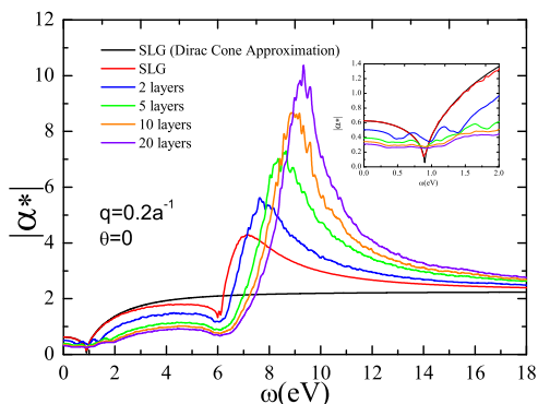
FIG. 15. (Color online) Modulus of the screened fine structure constant |\alpha^*| , calculated from Eq. (23), for SLG and MLG of a different number of layers. The inset is a zoom for the more experimentally relevant \omega \rightarrow 0 region of the spectrum (see text). |\alpha^*| \approx 0.6 for SLG, whereas this value is highly reduced for MLG: |\alpha^*| \approx 0.3 for a 20-layers sample in our numerical calculation, which has a behavior very similar to graphite.
