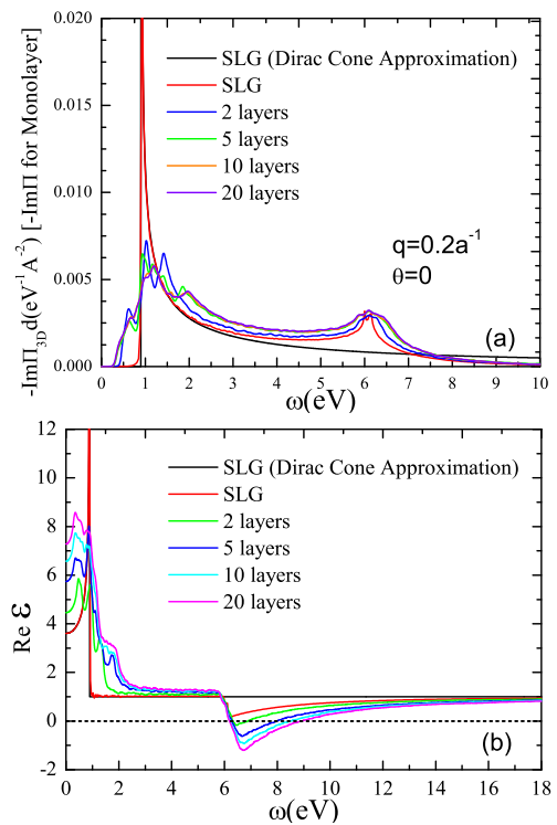
FIG. 11. (Color online) (a) \text{Im}\Pi(\mathbf{q}, \omega) for SLG and MLG. The results for SLG obtained from the Kubo formula Eq. (4) are compared to those obtained from the Lindhard function Eq. (11), and to the Dirac cone approximation. (b) \text{Re} \varepsilon(\mathbf{q}, \omega) for SLG and MLG, and comparison to the Dirac cone approximation, for the same value of q as in (a).
