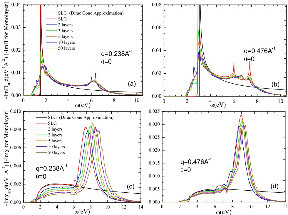
FIG. 14. (Color online) Non-interacting polarization function \text{Im}\Pi(\mathbf{q}, \omega) [plots (a) and (b)] and RPA response function \text{Im}\chi(\mathbf{q}, \omega) [plots (c) and (d)] for SLG and MLG, for two different wave-vectors. The wave-vectors are chosen as in Ref. 5.
