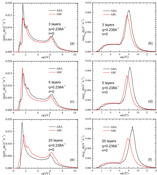
FIG. 10. (Color online) Dynamical polarization and response function of ABA- and ABC-stacked multilayer graphene. The number of layers are 3 layers in (a,b), 5 layers in (c,d) and 20 layers in (e,f). The size of each layer is 3600 \times 3600 atoms for tri-layer (a,b); 3200 \times 3200 atoms for 5-layer samples (c,d), and 1600 \times 1600 atoms for 20-layer (e,f).
