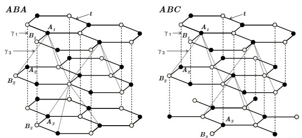
FIG. 1. Atomic structure of ABA- and ABC-stacked multi-layer graphene. The intra-layer ( t ) and inter-layer ( \gamma_1 and \gamma_3 ) hopping amplitudes are considered, as explained in the text.
