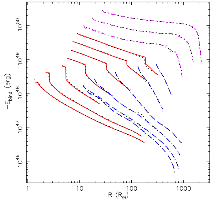
Figure 2. Envelope binding energy as a function of stellar radius, for a selection of models with masses of 0.91, 1.36, 2.04, 3.05, 4.57, 6.84, 10.22, 15.3, 22.9, and 34.2 M_{\odot} , and Z = 0.02 . The line styles and colors indicate the same evolutionary phases as in Figure 1 and are used for the results obtained by using our fit. The black dotted lines show the original stellar-evolution models, which overlap with the fits in most places. RGB and AGB phases are disconnected here, and the lowest-mass and the three highest-mass models do not have an AGB phase.
