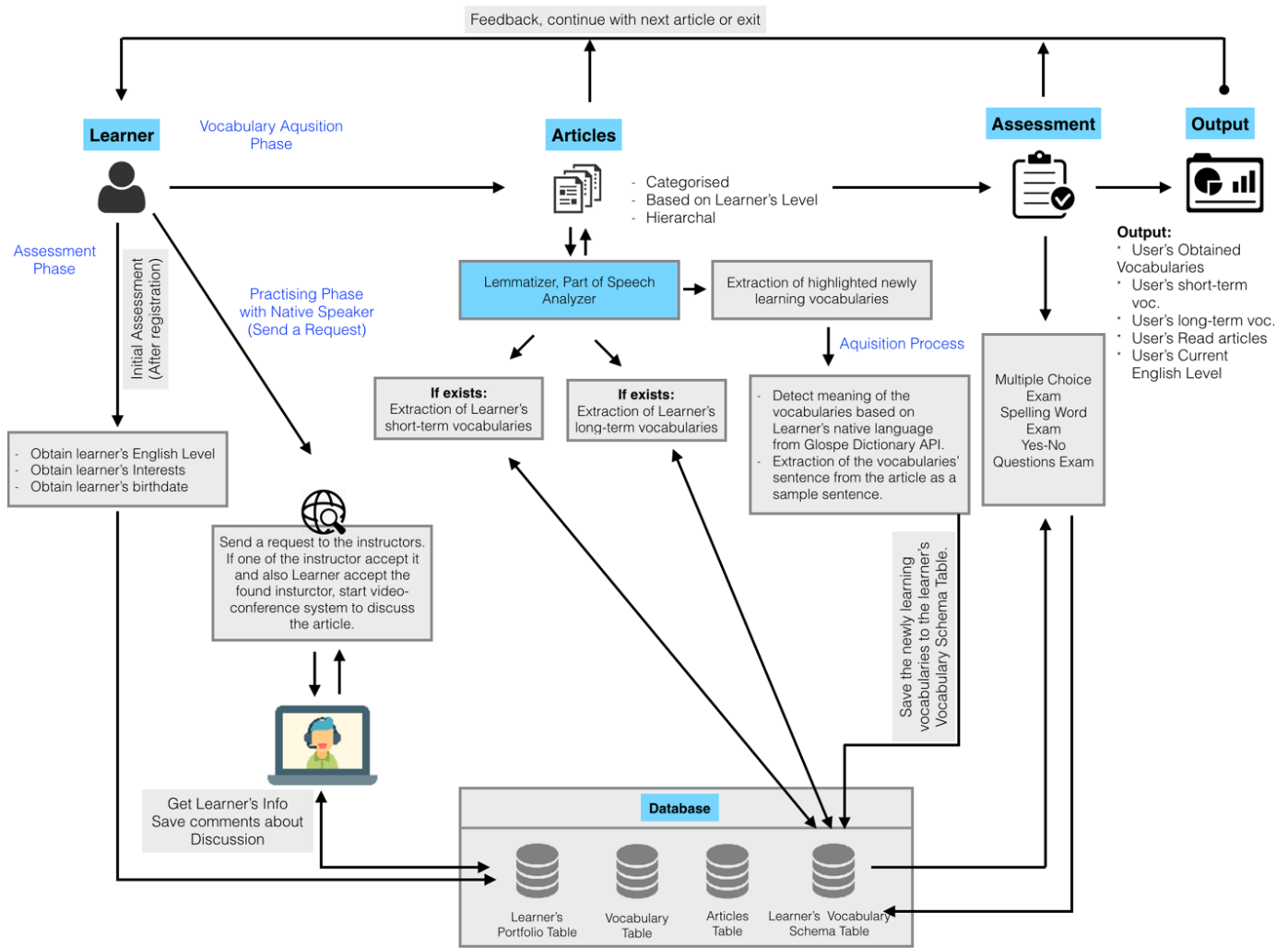
Figure 1: The Vocabulary Learning Processes of the System
