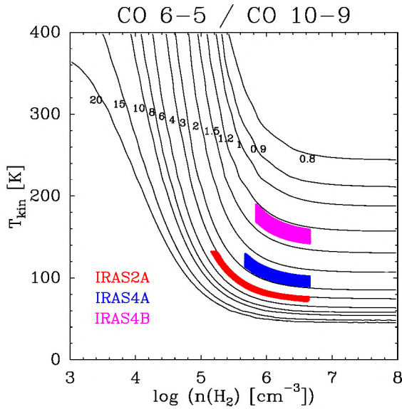
Fig. A.1. Model line ratios of CO 6–5/10–9 for a slab model with a range of temperatures and densities. The adopted CO column density is 10^{17} \text{cm}^{-2} with a line width of 10 \text{km s}^{-1} , comparable to the inferred values. For these parameters the lines involved are optically thin. The colored lines give the range of densities within the 20'' beam for the three sources based on the models of Jørgensen et al. (2002).
