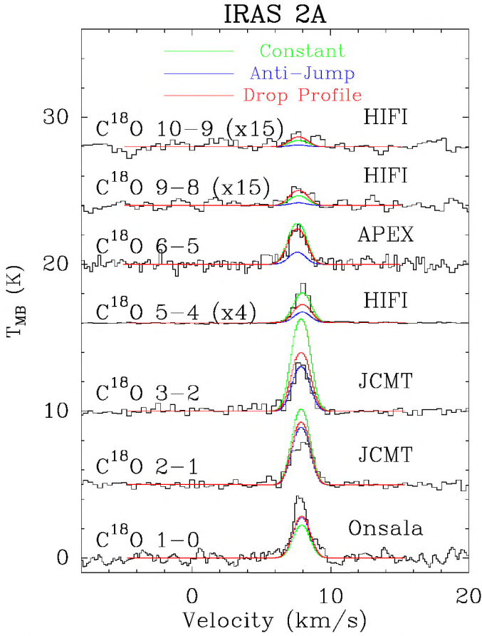
Fig. B.2. Best fit constant (green), anti-jump (blue) and drop abundance (red) Ratran models overplotted on the observed spectra. All spectra refer to single pointing observations. The calibration uncertainty for each spectrum is around 20–30% and is taken into account in the \chi^2 fit. See Table B.1 for parameters.
