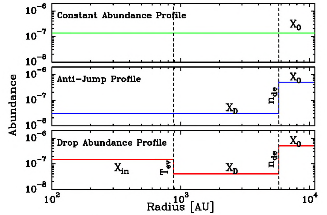
Fig. B.1. Examples of constant, anti-jump, and drop abundance profiles for IRAS 2A for T_{\text{ev}}=25 K and n_{\text{de}}=7 \times 10^4 \text{cm}^{-3}
