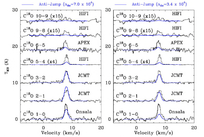
Fig. B.4. The IRAS 2A spectra for the X_0 and X_D parameters corresponding to the values in Jørgensen et al. (2005c) for different n_{\text{de}} values of 3.4 \times 10^4 and 7 \times 10^4 \text{ cm}^{-3} .
