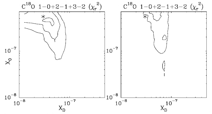
Fig. B.3. The \chi^2 plots for the anti-jump profiles where X_0 and X_D values are varied. Right: for n_{\text{de}} = 7 \times 10^4 and left: for n_{\text{de}} = 3.4 \times 10^4 \text{ cm}^{-3} . The asterisk indicates the value for Jørgensen et al. (2005c) used here. Contours are plotted at the 2\sigma , 3\sigma , and 4\sigma confidence levels ( left ) and 3\sigma and 4\sigma confidence levels ( right ).
