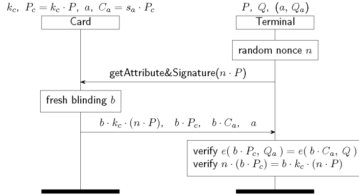
Figure 2. Optimised protocol for proving self-blindable attributes
