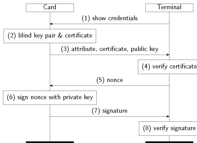
Figure 1. Sketch of the protocol
