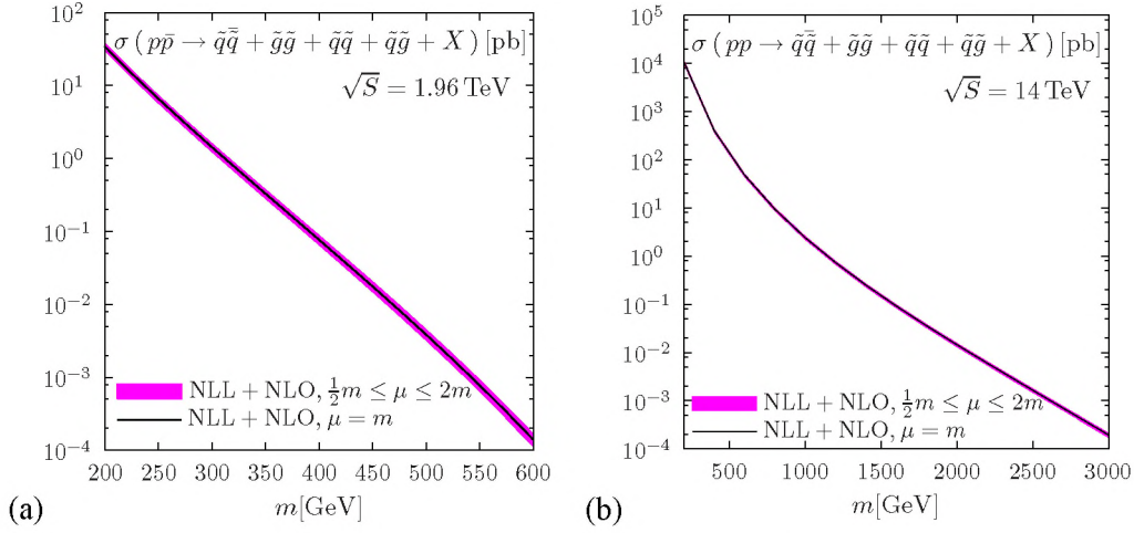
Figure 2: The NLL+NLO cross section for inclusive squark and gluino pair-production, p\bar{p}/pp \rightarrow \tilde{q}\bar{\tilde{q}} + \tilde{q}\tilde{q} + \tilde{q}\tilde{g} + \tilde{g}\tilde{g} + X , at the Tevatron (a) and the LHC (b) as a function of the average particle mass m . Shown are results for the mass ratio r = m_{\tilde{g}}/m_{\tilde{q}} = 1 . The error band corresponds to a variation of the common renormalization and factorization scale in the range m/2 \leq \mu \leq 2m .
