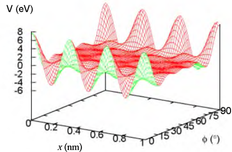
FIG. 2. An example of the shape of V(x, \phi) as obtained from the potential V_A(x, y) in Eq. (15) at constant y and z , summed over the atoms of a nanocrystal with square contact layer of 4 \times 4 unit cells (and therefore 5 \times 5 atoms) with lattice parameter 0.31585 nm on a square lattice with corrugation V_1 = 1 eV and V_2 = V_3 = V_1/2 and lattice parameter 0.32668 nm. These parameters correspond to W(001) and NaF(001).
