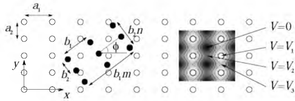
FIG. 4. A top view of a general rectangular lattice (open circles) and contact layer (filled circles) with mismatch angle \phi , lattice parameters a_1, a_2, b_1, b_2 , contact layer size m, n , and the potential energy of a contact layer atom on the substrate. If a contact layer atom lies on top of a substrate atom, its potential energy is V_1 . If it lies directly between an atom and its nearest neighbour in the x or y direction, it has potential energy V_2 or V_3 respectively. If it lies in the centre of a rectangle, at equal distance from four substrate atoms, without loss of generality, we may set the potential energy to 0. The origin of the coordinate system is chosen to lie on top of a substrate atom.
