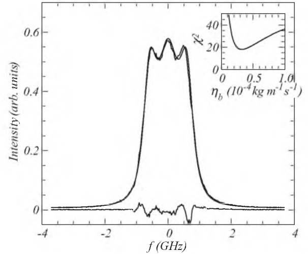
FIG. 6. \text{SF}_6 spontaneous Rayleigh-Brillouin scattering at p = 1.95 bar compared to the Tenti S6 model, which was computed taking \eta_b = 3.5 \times 10^{-5} \text{ kg m}^{-1} \text{ s}^{-1} . Lower full line shows the difference between experiment and the Tenti S6 model. Inset shows the \chi^2 error as a function of \eta_b . In this experiment, the sound frequency is f = 575 MHz, which follows from c_{\text{int}} = 3/2 and the scattering wave vector k = 2.42 \times 10^7 \text{ m}^{-1} .
