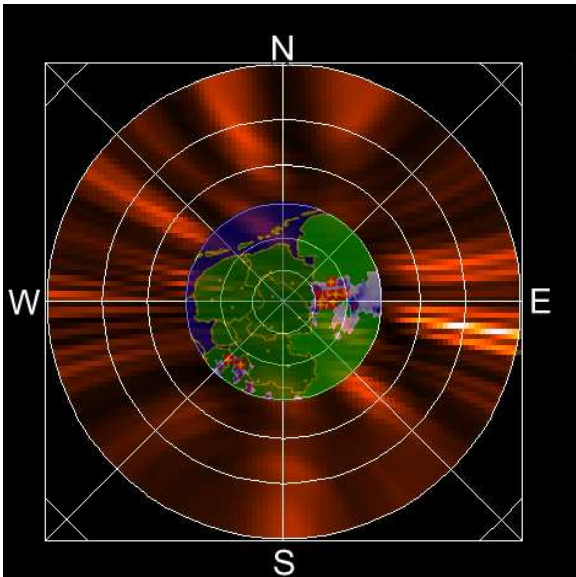
Figure 3: Terrestrial lightning as observed with buienradar (inner part) and LOFAR (outer part).
