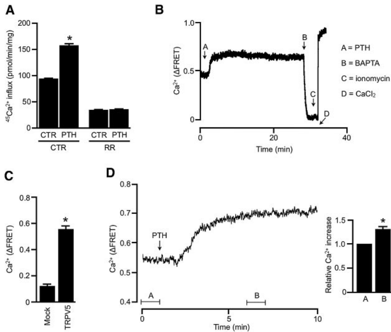
Figure 1. PTH rapidly induces a sustained stimulation of TRPV5-mediated \text{Ca}^{2+} influx. (A) ^{45}\text{Ca}^{2+} influx in HEK293 cells transiently coexpressing PTH1R and TRPV5, pretreated for 30 min with 25 \mu\text{M} BAPTA-AM. All procedures were performed at 37°C, and PTH or DMSO solvent (CTR) was administered simultaneously with ^{45}\text{Ca}^{2+} . * P < 0.05 versus CTR. TRPV5-specific ^{45}\text{Ca}^{2+} influx was determined by addition of 10 \mu\text{M} ruthenium red (RR). (B) Representative trace of intracellular \text{Ca}^{2+} upon PTH stimulation using yellow cameleon 2.1 as a FRET sensor. (C) Basal calibrated \text{Ca}^{2+} levels in HEK293 cells transfected with mock ( n = 8 ) and TRPV5 ( n = 9 ). * P < 0.05 versus mock. (D) Average trace of intracellular \text{Ca}^{2+} levels of TRPV5 upon treatment with PTH ( n = 9 ). (Inset) Relative FRET \text{Ca}^{2+} increase from basal to PTH-stimulated conditions, as shown by time periods "A" and "B," respectively. *Significant difference ( P < 0.05 ) from basal conditions.
