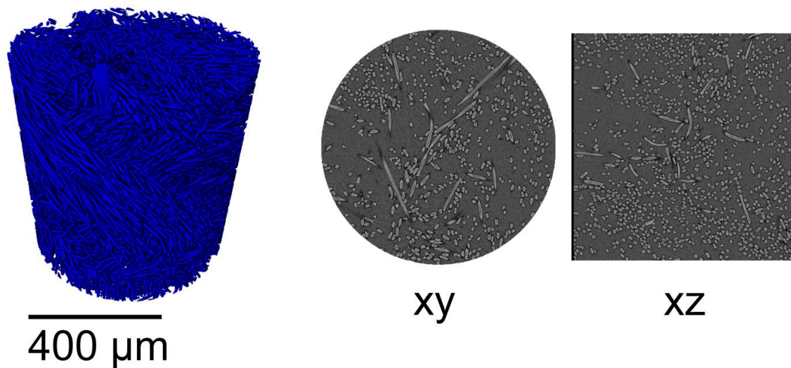
Figure 4 3D rendering (left) and orthoslices (right) of the ex situ felt after compression, shown here for the 20\times scan. No significant change in the fibre morphology or microstructure is seen, though an inelastic deformation of the bulk felt occurs on compression, reducing the porosity of the sample to 85%.
