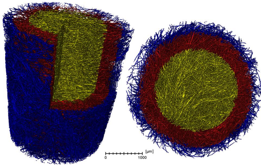
Figure 8 Radial porosity of the felt at 0% (black), 25% (red), 50% (blue), 75% (pink) and 90% (green) compression taken from the volume fraction of the outer (blue), middle (red) and inner (yellow) regions of the volume, indicated by the 3D rendering of the 0% compression 4 \times scan in the top half of the figure ( xz , left, and xy ,
