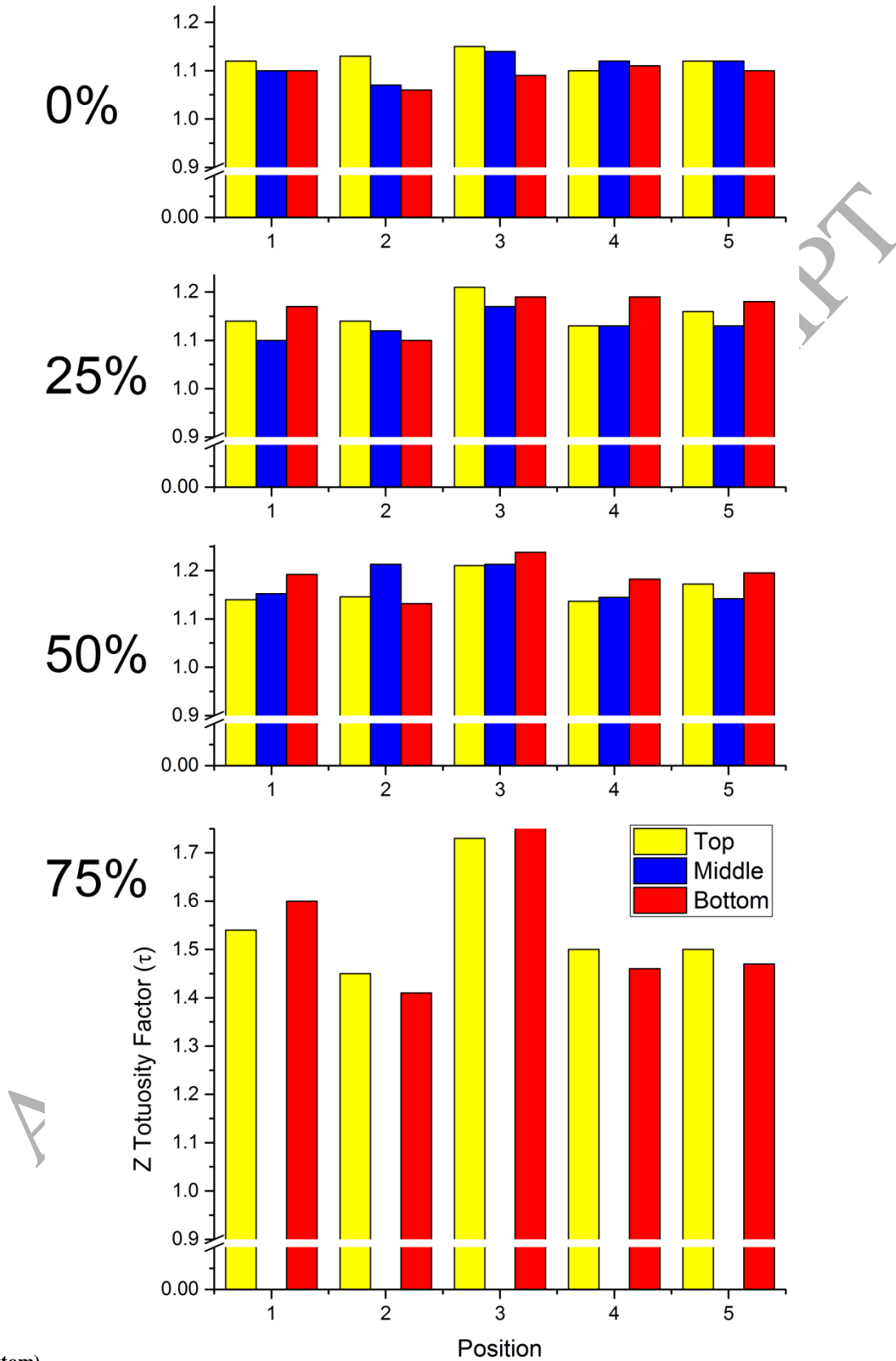
Figure 14 Tortuosity factor in the z-direction for all the locations of the 300^3 voxel sub-volumes shown in Figure 13 (positions 1-5 and top (yellow), middle (blue) and bottom (red)) for compressions 0% - 75% (top to
