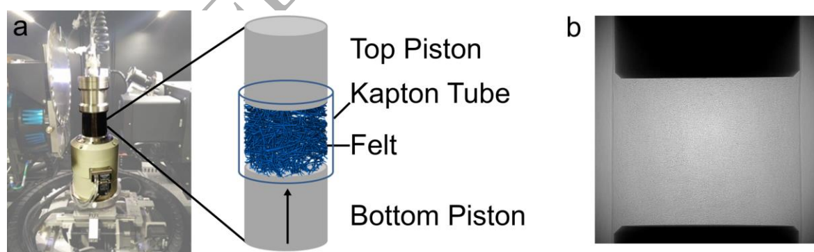
Figure 1 The experimental set up showing the compression rig in the CT machine (a) and an X-ray radiograph of the felt at 50% compression, fully in the field-of-view of the scan with 4\times magnification (b).
