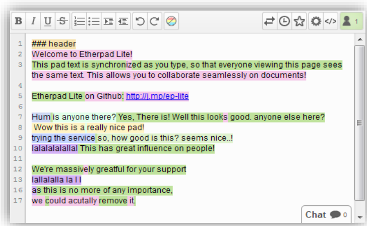
Figure 3 14 Etherpad
