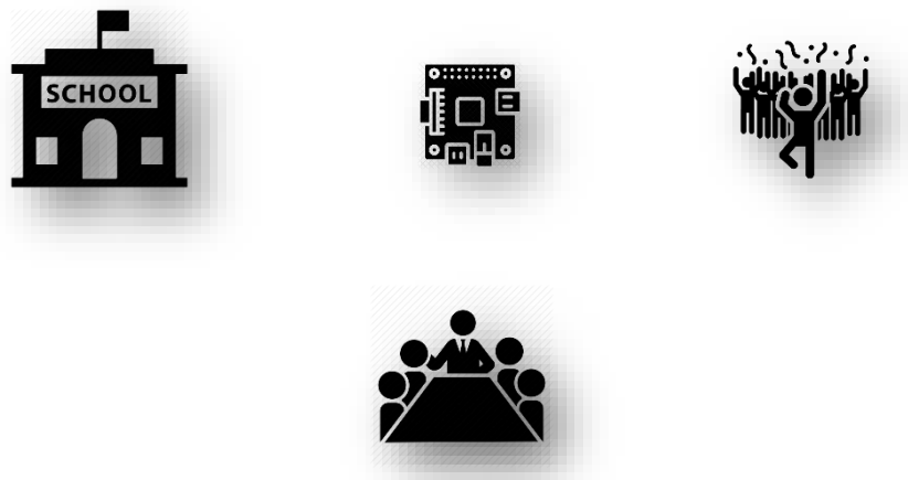
Figure 3 8 uses cases
