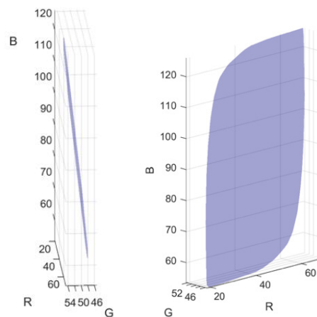
Figure 1: Two views of the very thin metamer mismatch body (MMB) found for the Point Grey Grasshopper2 camera
