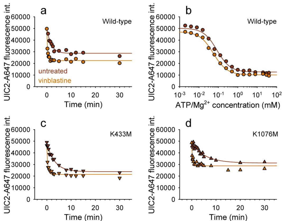
Figure 3. Kinetics of the formation of the BeF x -trapped species in case of wild-type (a) and single mutant (c,d) Pgp expressing cells. Permeabilized cells were incubated with 100 μM (for wild-type) or 500 μM (for K433M and K1076M) ATP/Mg 2+ and BeF x (200 μM BeSO 4 and 1 mM NaF) in the presence or absence of 50 μM vinblastine at 37°C and samples were taken at different time points. Panel (b) shows the effect of 200 μM vinblastine on the apparent nucleotide affinity of wild-type Pgp. Permeabilized cells were treated with BeF x and different concentrations of ATP/Mg 2+ in the presence or absence of 200 μM vinblastine for 20 min at 37°C. UIC2-A647 labeling was carried out following the washout of ATP/Mg 2+ in the maintained presence of BeF x .
