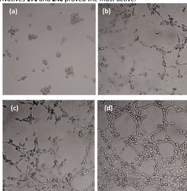
Fig. 3. Effect of compound 24c at 5 \mu\text{M} (a), 0.5 \mu\text{M} (b), 0.05 \mu\text{M} (c) and 0.025 \mu\text{M} (d) concentrations.
