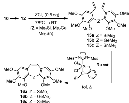
Scheme 7 Synthesis of tricyclic derivatives
