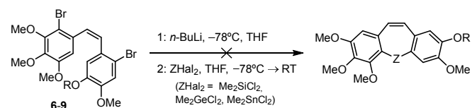
Scheme 3 Attempts to prepare tricyclic derivatives
