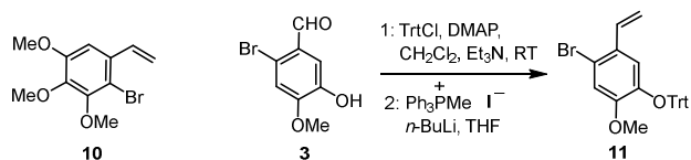
Scheme 5. Structure of 10 and synthesis of 11
