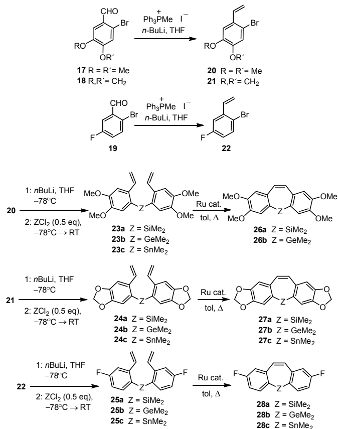
Scheme 8 Synthesis of tricyclic derivatives
