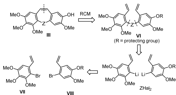
Scheme 4 Retrosynthetic analysis based on RCM
