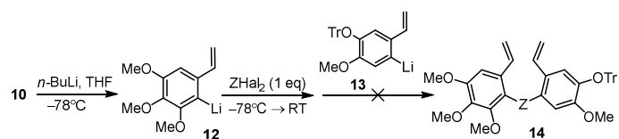
Scheme 6 Attempts to prepare 14
