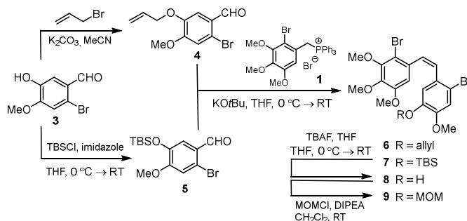
Scheme 2 Synthesis of dibromo derivatives 6–9 . Abbreviations: TBS, tert -butyldimethylsilyl; TBAF, tetra- n -butylammonium fluoride; MOM, methoxymethyl; DIPEA, N,N -diisopropyl ethylamine.
