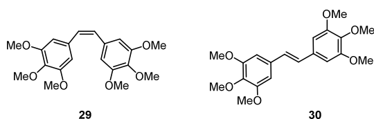
Scheme 9 Structures of ( Z ) and ( E )-1,2-bis(3,4,5-trimethoxyphenyl) ethylene
