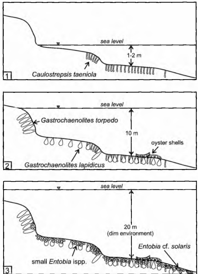
Fig. 8. Succession of borings (from 1 do 3) in relation to changing water depth during a single transgressive cycle of the 4 th order (example from the Miocene regional transgression in the Mut Basin, southern Turkey). The borings and proportions not to the scale
