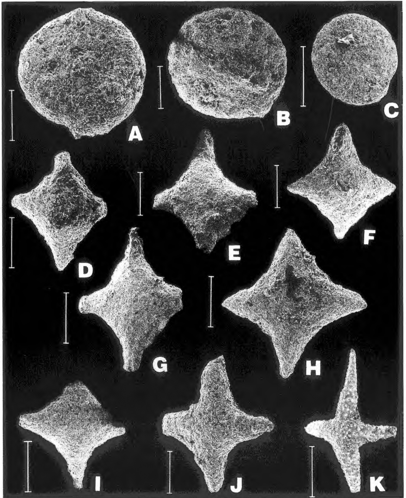
Fig. 7. SEM micrographs of Spumellaria. A-C. Orbiculiforma sp.; D-K. Crucella theokaftensis Baumgartner. Length of scale bar – 100 \mu\text{m}
