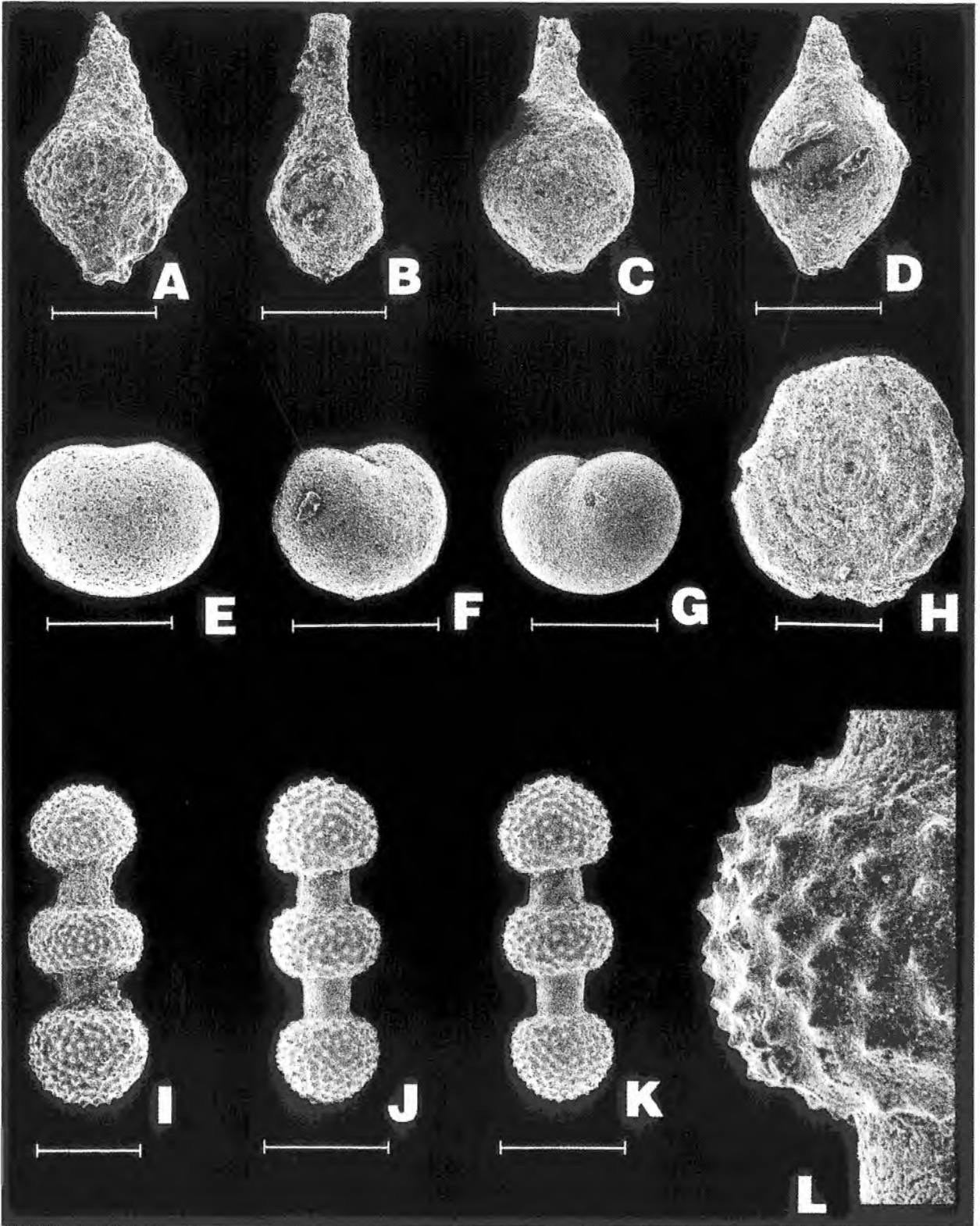
Fig. 10. SEM micrographs of Nassellaria, Foraminifera and sponge spicules. A-C. Syringocapsa vicetina (Squinabol); D. Syringocapsa sp.; E-G. Rhax ; H. Spirillina gracilis Terquem; I-L. Criccorhabd. Length of scale bar – 100 \mu\text{m}
