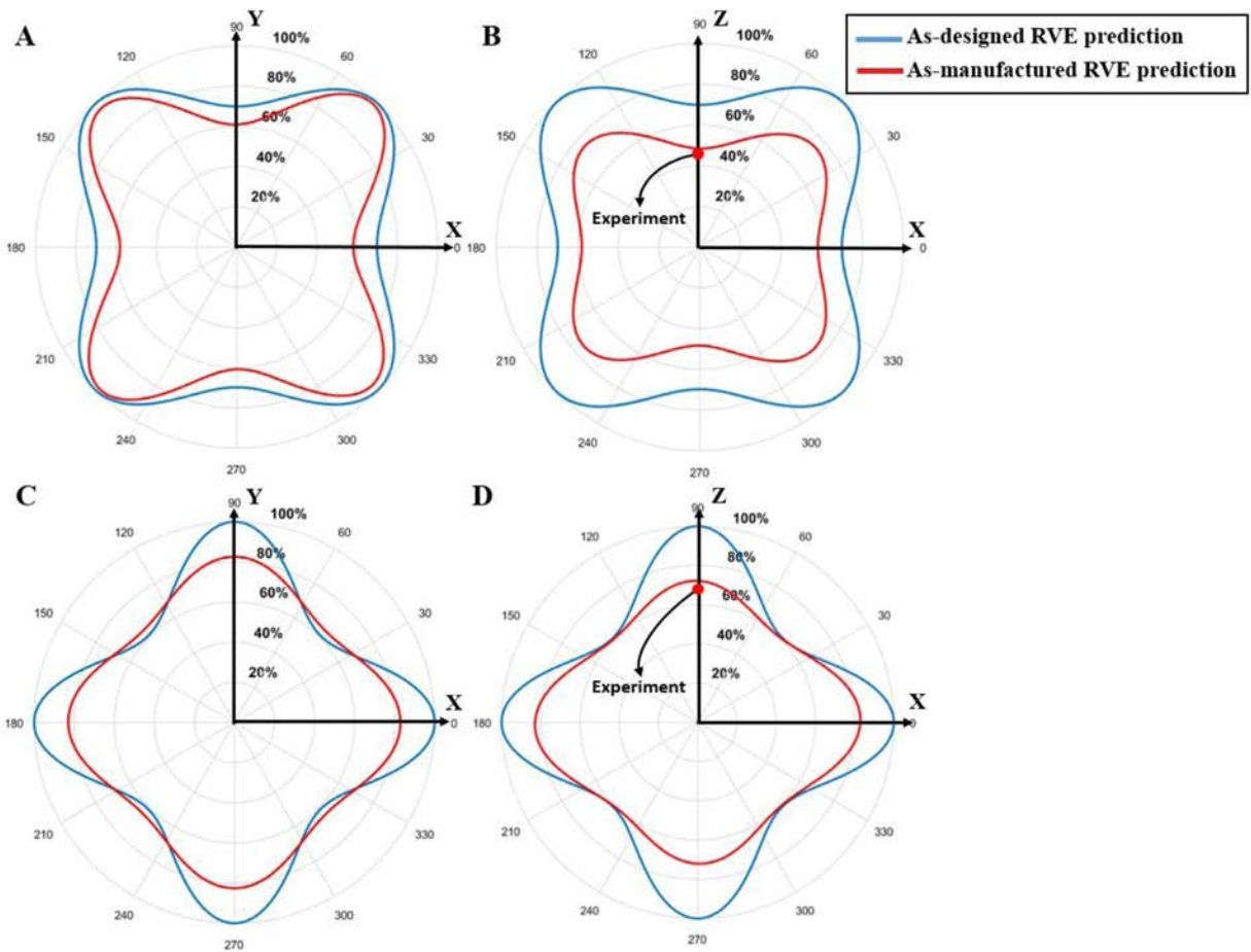
Fig. 11. Polar plots illustrating the variation of the normalized Young's modulus for the as-designed, and CT reconstructed representative volume elements:
