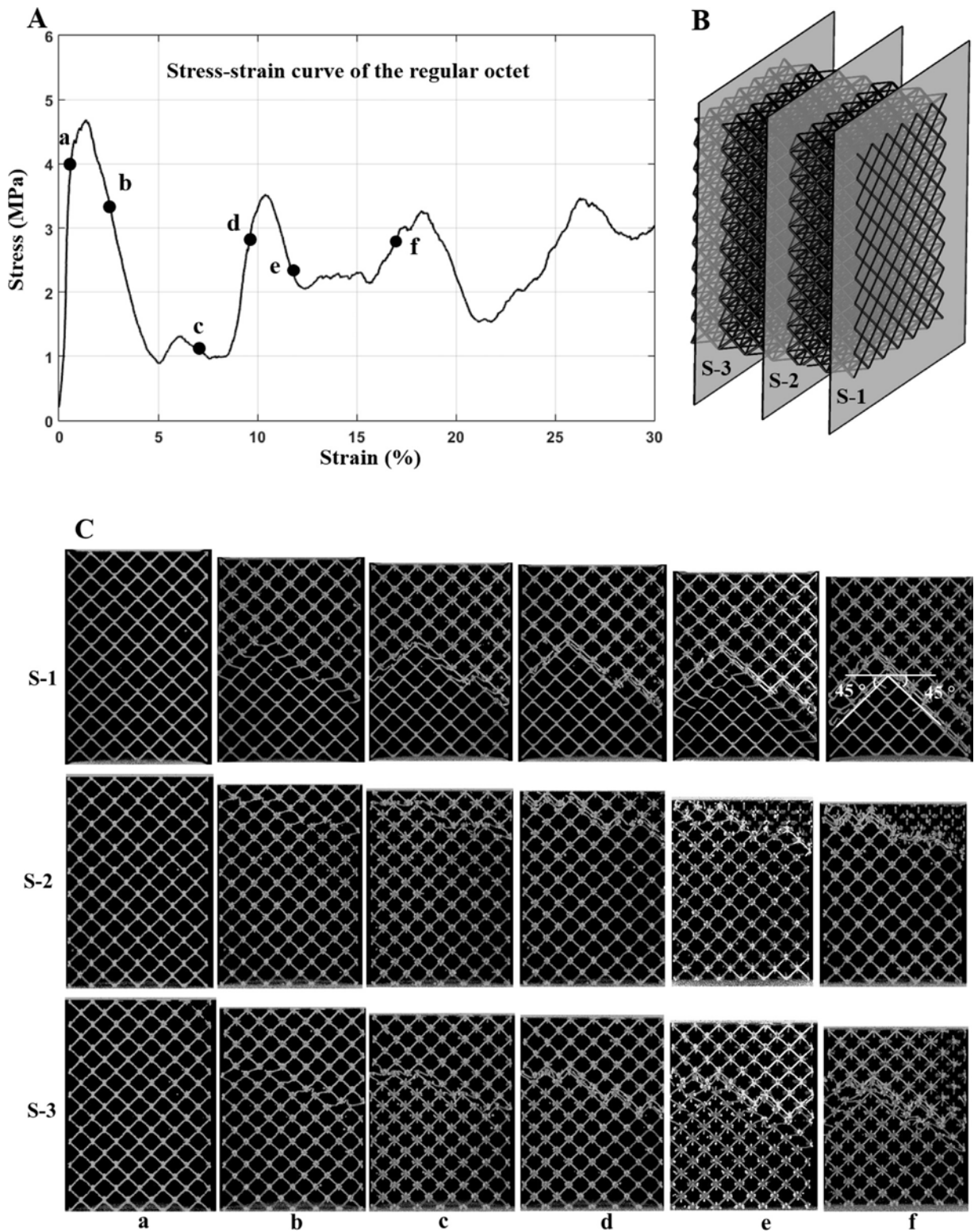
Fig. 7. CT in-situ compression images for a representative regular
