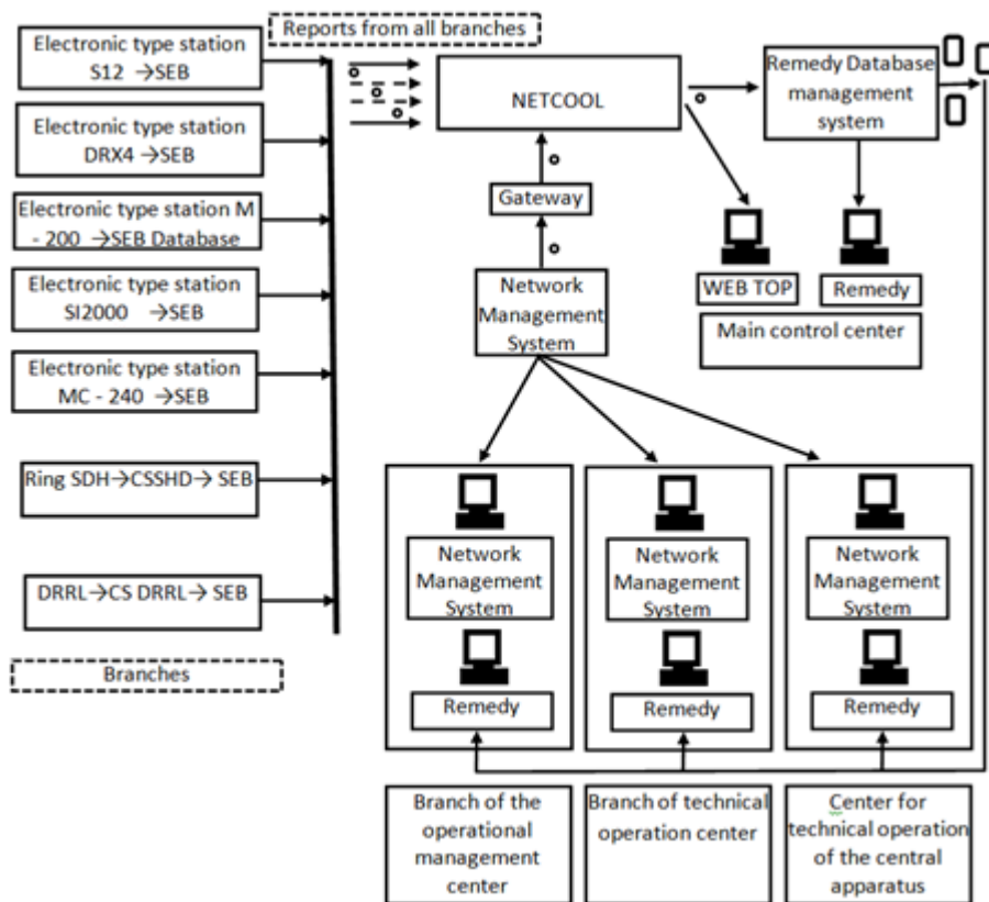
Fig. 4. Interaction Pattern: Network Management System - NETCOOL – PTMS (REMEDY).
