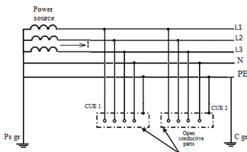
Fig. 2 Diagram of an electrical network with TN-S neutral grounding system.
