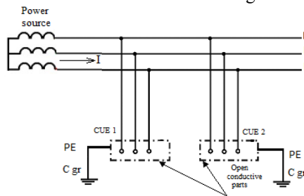
Fig. 5 Diagram of an electrical network with IT neutral grounding system.
