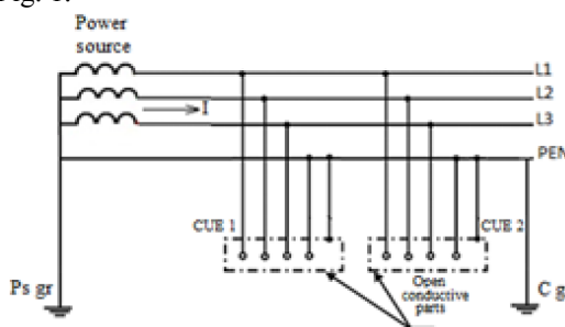
Fig. 1 Diagram of an electrical network with TN-C neutral grounding system.
