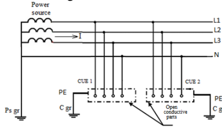
Fig. 4 Diagram of an electrical network with TT neutral grounding system.
