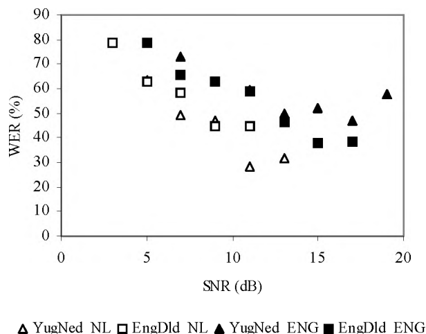
Figure 2: WERs for different SNR values.
