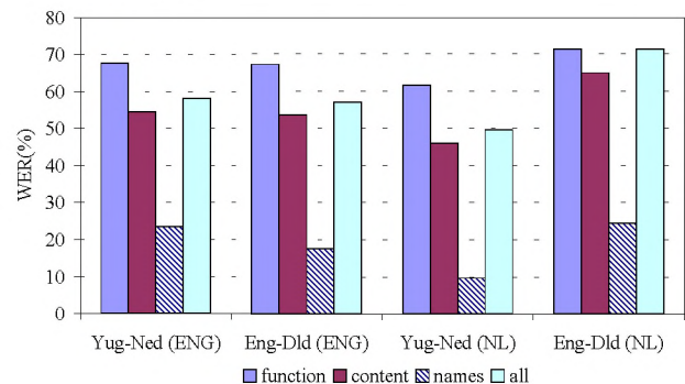
Figure 1: WERs according to word type.
