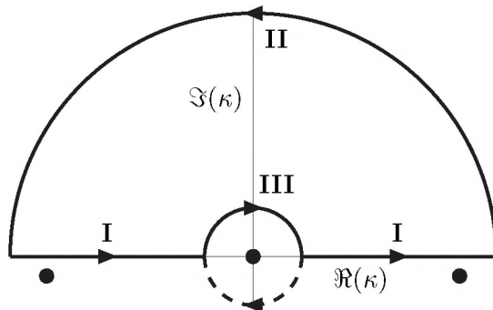
Figure 1: Principle value integral
