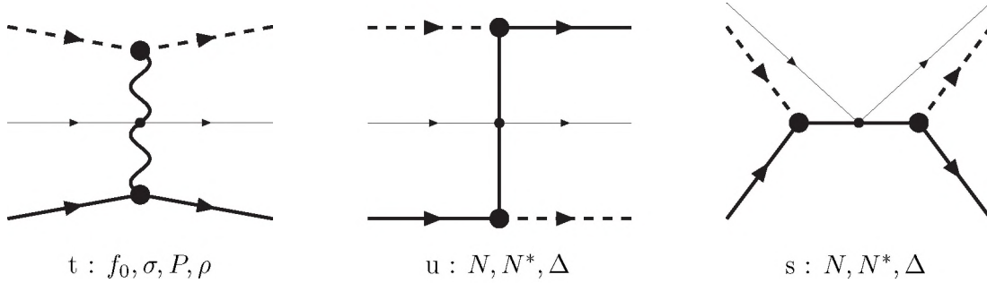
Figure 2: Tree level amplitudes as input for integral equation. The inclusion of the quasi particle lines is schematically. Therefore, the diagrams represent either the (a) or the (b) diagram.
