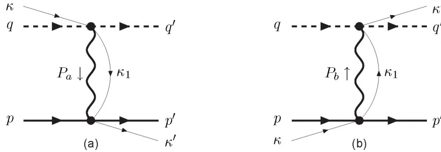
Figure 4: Vector meson exchange in Kadyshevsky formalism.
