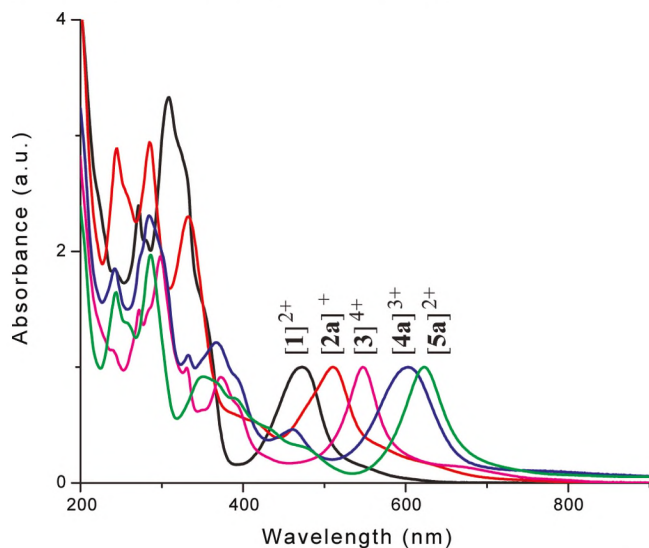
Figure 3. Electronic absorption spectra of [1]^{2+} , [2a]^+ , [3]^{4+} , [4a]^{3+} , and [5a]^{2+} in MeCN.
