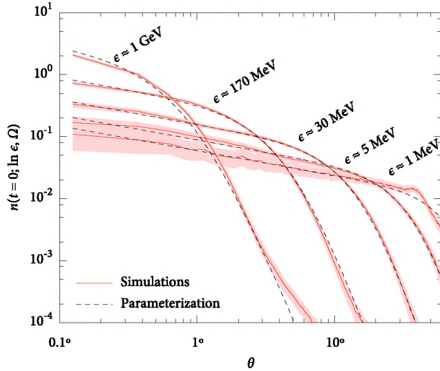
Fig. 5. Normalised average electron distributions n(t=0; \ln \epsilon, \Omega) (solid) for 20 proton showers at 10^{18} eV with 3\sigma statistical error margins (filled area). For each energy, corresponding parameterizations according to (8) are also drawn (dashed).
