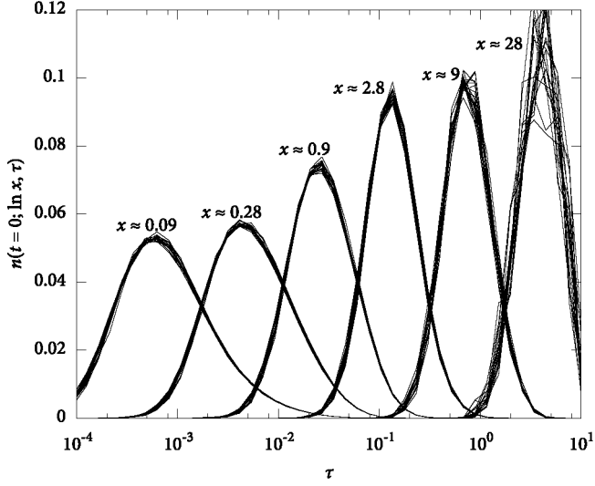
Fig. 18. Electron distributions n(t=0; \ln x, \tau) as a function of particle time lag for 20 individual showers initiated by 10^{19} eV protons.
