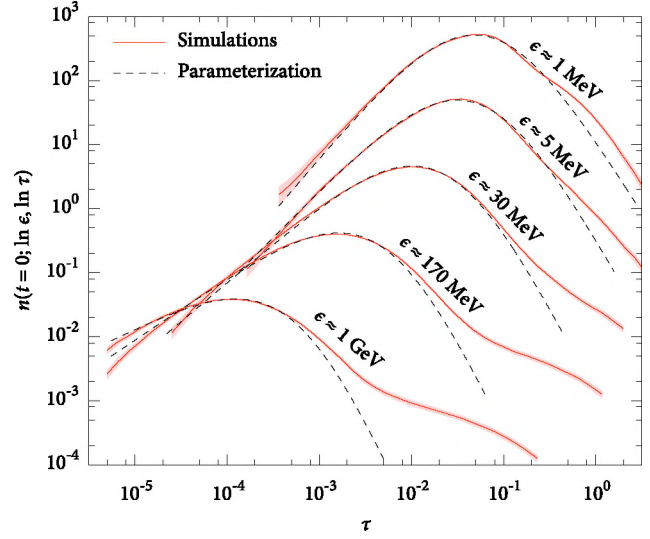
Fig. 17. Normalised average electron distributions n(t = 0; \ln \epsilon, \ln \tau) (solid) for 20 proton showers at 10^{19} eV with 3\sigma statistical error margins (filled area). For each energy, corresponding parameterizations according to (16) are also drawn (dashed). Consecutive sets are again shifted up by a factor of 10.
