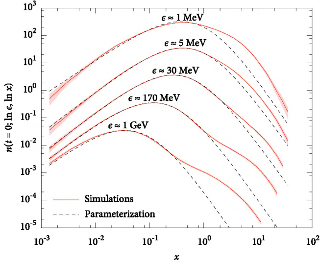
Fig. 13. Normalised average electron distributions n(t=0; \ln \epsilon, \ln x) (solid) for 20 proton showers at 10^{18} eV with 3\sigma statistical error margins (filled area). For each energy, corresponding parameterizations according to (14) are also drawn (dashed). Consecutive sets are again shifted up by a factor of 10.
