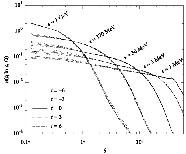
Fig. 4. Normalised average distributions n(t; \ln \epsilon, \Omega) for different shower stages, averaged over 20 proton-initiated showers at 10^{18} eV.
