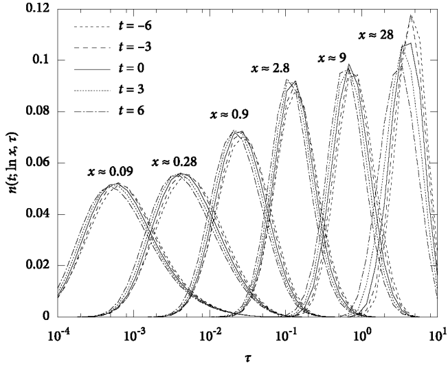
Fig. 19. Average distributions n(t; \ln x, \tau) for different evolution stages, averaged over 20 proton-initiated showers at 10^{19} eV.
