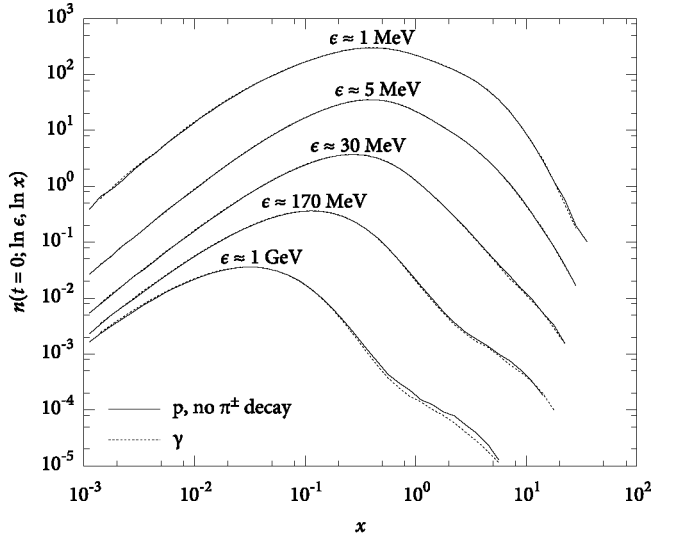
Fig. 12. Comparison of average distributions n(t = 0; \ln \epsilon, \ln x) at 10^{17} eV for 20 standard photon showers to 20 proton showers in which \pi^\pm decay was disabled. Again, consecutive sets are shifted up by a factor of 10.
