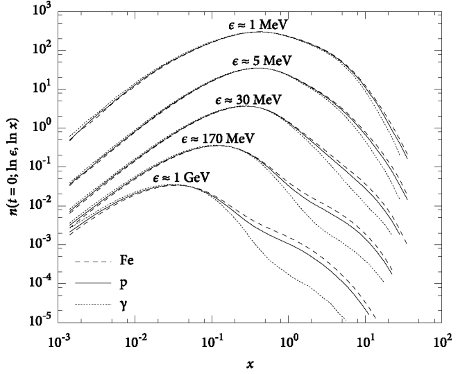
Fig. 11. Average distributions n(t = 0; \ln \epsilon, \ln x) for different primaries, averaged over 20 showers at 10^{18} eV. Again, consecutive sets are shifted up by a factor of 10. Note the dependence on species of the bulge on the right.
