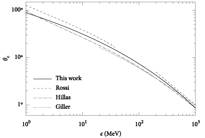
Fig. 6. Cutoff angle \theta_c according to (9) for the angular distribution as a function of secondary energy (solid line). Also shown are theoretical predictions for \theta_{\text{RMS}} from Rossi & Greisen [3] (dashed) as well as empirical relations from Hillas [5] (dash-dotted) and Giller et al. [6] (dotted).
