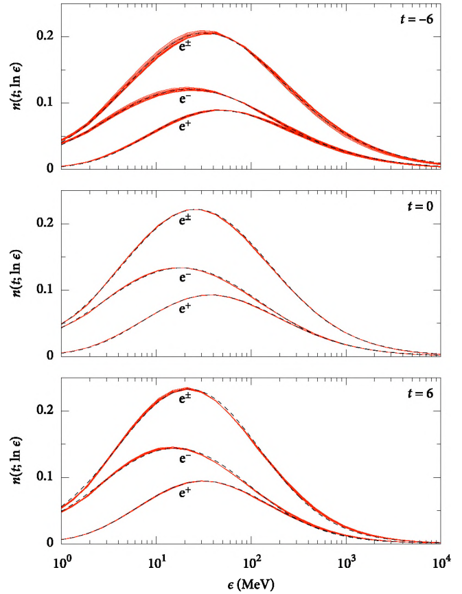
Fig. 2. Average energy distribution for different evolution stages t = -6, 0, 6 for electrons (marked e^- ), positrons ( e^+ ), and their sum ( e^\pm ). Background curves represent simulated distributions for different primaries (p, Fe, and \gamma ) and energies ( 10^{17} , 10^{18} and 10^{19} eV). The corresponding parameterized distributions from (6) are plotted on top (dashed).
