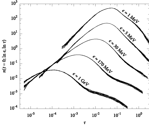
Fig. 15. Electron distributions n(t = 0; \ln \epsilon, \ln \tau) for different electron energies as a function of delay time for 20 individual showers initiated by 10^{19} eV protons. The curve set for 1 GeV is at the actual level; consecutive sets are shifted up by a factor of 10.
