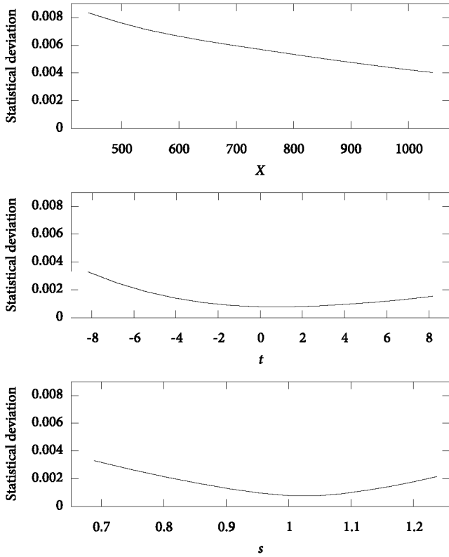
Fig. 1. Average statistical deviation from the average energy distribution for 180 air showers of different energy and primary species, averaged in slant depth (top), relative evolution stage (middle), and age (bottom). On average, the longitudinal range is the same in each plot.
