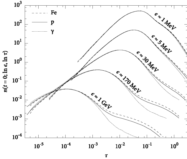
Fig. 16. Average distributions n(t = 0; \ln \epsilon, \ln \tau) for different primaries, averaged over 20 showers at 10^{19} eV. Consecutive sets are again shifted up by a factor of 10. Note the species-dependent bulge on the right as in Fig. 11.
