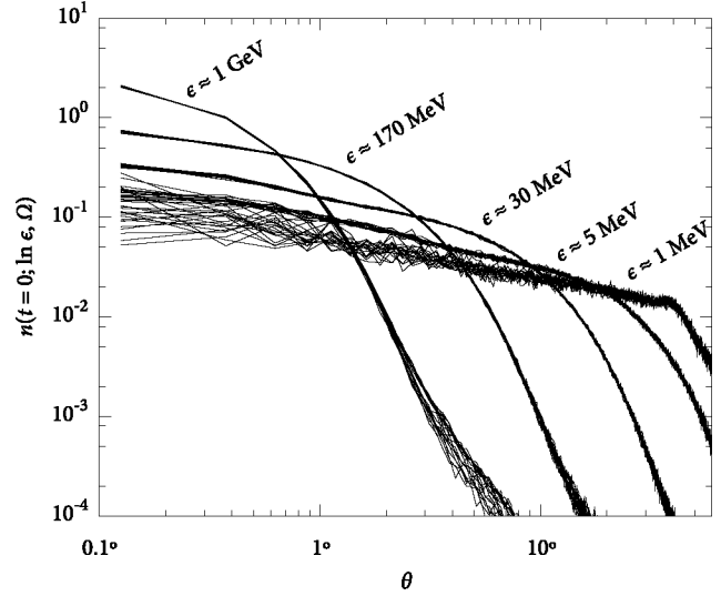
Fig. 3. Electron distributions n(t=0; \ln \epsilon, \Omega) at different electron energies as a function of momentum angle to the shower axis for 20 individual showers initiated by 10^{18} eV protons. 0^\circ is along the primary's trajectory, 90^\circ is perpendicular to the shower axis.
