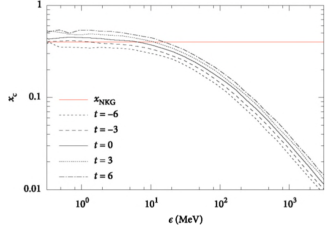
Fig. 14. Cutoff distance x_c as a function of secondary energy at different shower stages. The energy-independent overall break distance obtained from the NKG function is also plotted (horizontal line).
