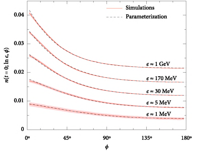
Fig. 8. Normalised average electron distributions n(t = 0; \ln \epsilon, \phi) (solid) for 20 proton showers at 10^{18} eV with 3\sigma statistical error margins (filled area). For each energy, corresponding parameterizations according to (10) are also drawn (dashed).
