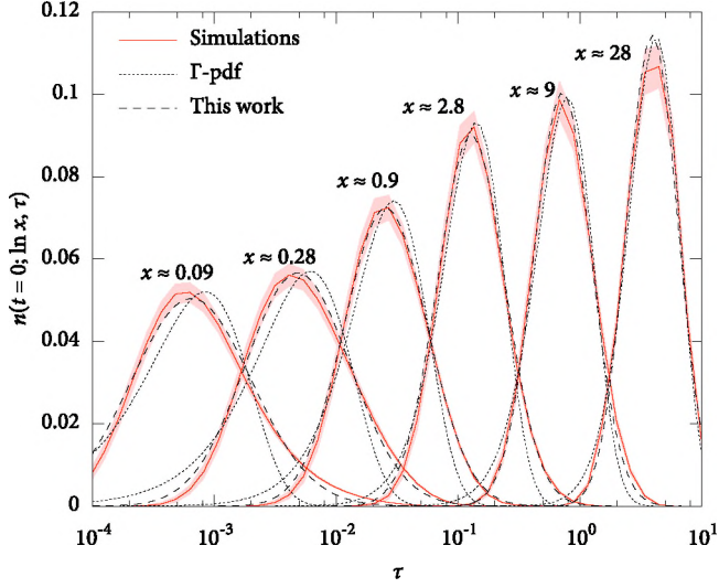
Fig. 21. Average electron distributions n(t=0; \ln x, \tau) (solid) for the reference set with 3\sigma statistical error margins (filled area). For each distance, corresponding parameterizations according to (18) are drawn as well (dashed). Best-fit \Gamma -pdf are also plotted (dotted).
