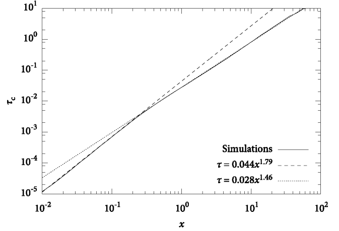
Fig. 22. Maximum density \tau_c as a function of lateral distance x at the shower maximum. Also shown are curves for x < x_0 (dashed) and x > x_0 (dotted) according to the parameterization in (21).
