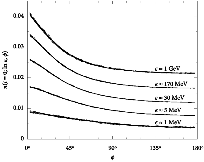
Fig. 7. Normalised simulated horizontal angular electron distributions for 20 individual showers initiated by 10^{18} eV protons at different energies. Consecutive curve sets are shifted up by 0.005 to distinguish them better; curves for 1 MeV are at the actual level.
