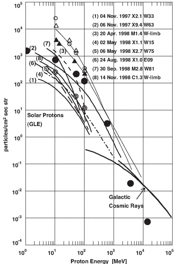
Figure 4. Integral flux of solar protons. Black dots represent the 2001 Easter event, for details see [59,60].
