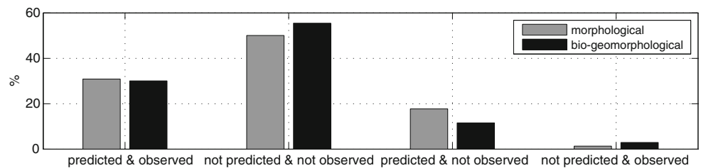
Fig. 12 Results for the morphological case and bio-geomorphological case, evaluated against observed sand wave occurrence in the Dutch part of the North Sea
