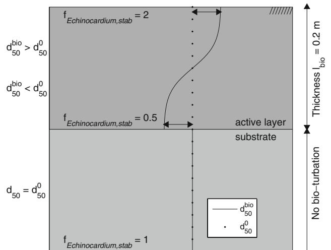
Fig. 5 Schematic overview of the influence of Echinocardium cordatum on the grain size distribution in the bed. Resulting in a larger grain size in the surface layer and a smaller grain size in the subsurface layer ( d_{50}^{bio} ), compared to the physical case ( d_{50}^0 ), expressed in a stabilization factor ( f_{Echinocardium,stab} ). In the substrate, no bio-turbation occurs
