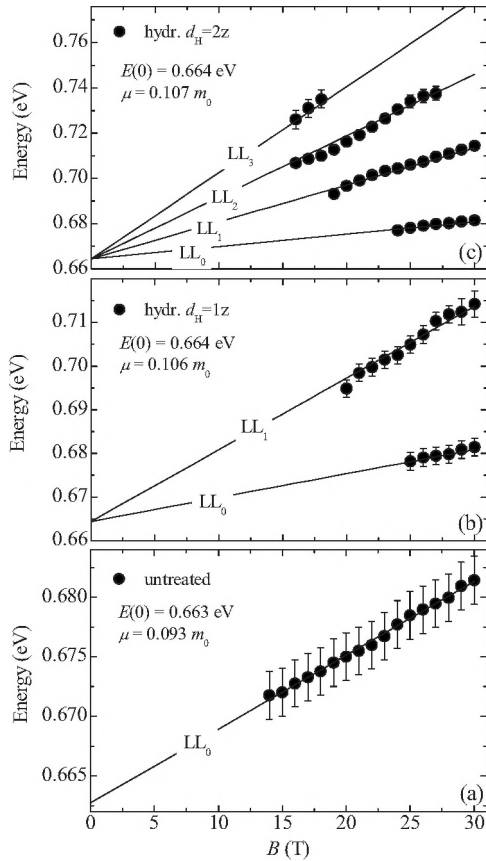
FIG. 3. Energies of the LL_n transitions highlighted in Fig. 2 as a function of the magnetic field. (a) refers to the untreated (as-grown) sample. (b) and (c) refer, respectively, to samples hydrogenated with d_H=1z and d_H=2z ( z=10^{15} \text{ cm}^{-2} ). Lines are fits to the data by Eq. (1), where the value of the band-gap energy at B=0 T, E(0) , and the value of the carrier reduced mass \mu are used as fit parameters for each sample separately.
