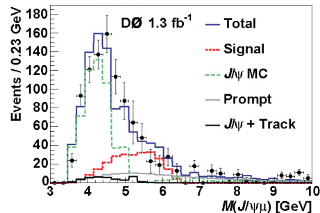
FIG. 1: Fit to the mass of the J/\psi + \mu vertex with J/\psi mass sideband and B^+ components subtracted and decay length significance L_{xy}/\sigma(L_{xy}) > 4 required. (color online)
