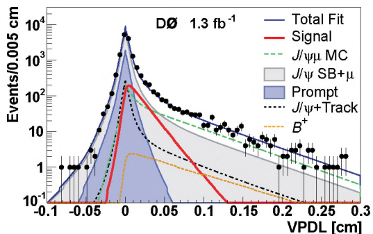
FIG. 2: VPDL distribution of the J/\psi\mu sample with the projected components of the fit overlaid. (color online)
