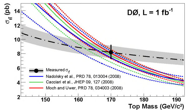
FIG. 2: Experimental and theoretical [1, 2, 3] \sigma_{t\bar{t}} as function of m_t . The colored dashed lines represent the theoretical uncertainties due to the choice of the PDF and the renormalization and factorization scales. The point shows the measured combined \sigma_{t\bar{t}} , the black dashed line the fit with Eq. 4 and the gray band the corresponding total experimental uncertainty.
