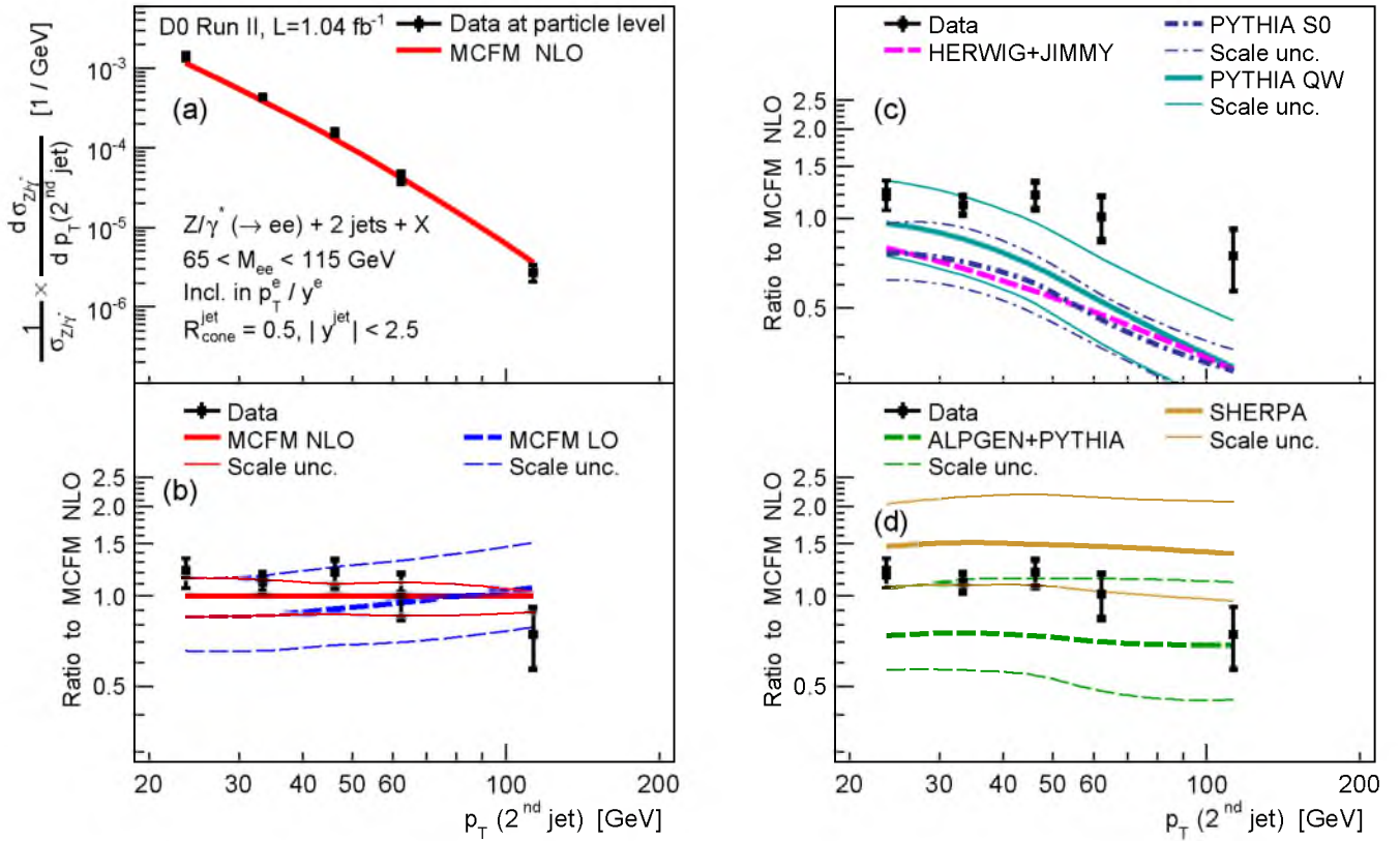
FIG. 2: (a) The measured distribution of \frac{1}{\sigma_{Z/\gamma^*}} \times \frac{d\sigma}{dp_T(\text{2nd jet})} for the second jet in Z/\gamma^* + 2 \text{ jets} + X events, compared to the predictions of MCFM NLO. The ratios of data and theory predictions to MCFM NLO are shown (b) for pQCD predictions corrected to the particle level, (c) for three parton-shower event generator models, and (d) for two event generators matching matrix-elements to a parton shower. The scale uncertainties were evaluated by varying the factorization and renormalization scales by a factor of two.
