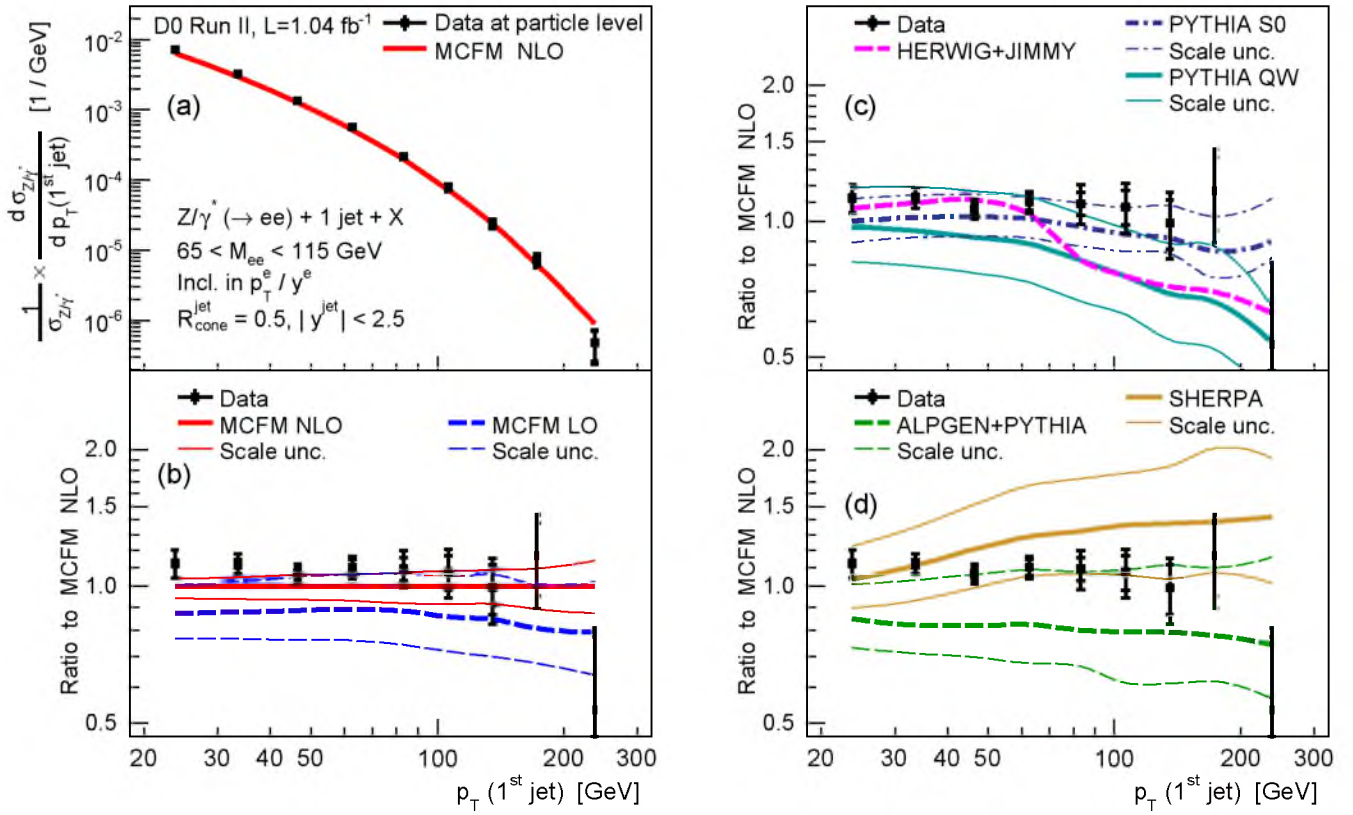
FIG. 1: (a) The measured distribution of \frac{1}{\sigma_{Z/\gamma^*}} \times \frac{d\sigma}{dp_T(\text{1st jet})} for the leading jet in Z/\gamma^* + \text{jet} + X events, compared to the predictions of MCFM NLO. The ratios of data and theory predictions to MCFM NLO are shown (b) for pQCD predictions corrected to the particle level, (c) for three parton-shower event generator models, and (d) for two event generators matching matrix-elements to a parton shower. The scale uncertainties were evaluated by varying the factorization and renormalization scales by a factor of two.
