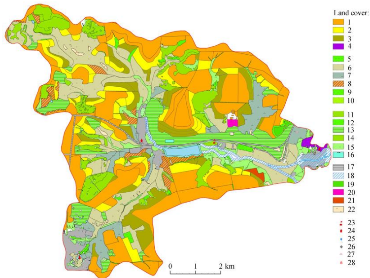
Figure 2: The results of designing a basin-based organization of nature management for one of the small river basin.
