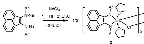
Ar = 2,6- \text{iPr}_2\text{C}_6\text{H}_3 Scheme 2. Synthesis of 2 .
