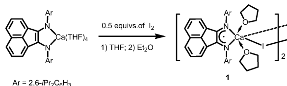
Ar = 2,6- \text{iPr}_2\text{C}_6\text{H}_3 Scheme 1. Synthesis of 1 .
