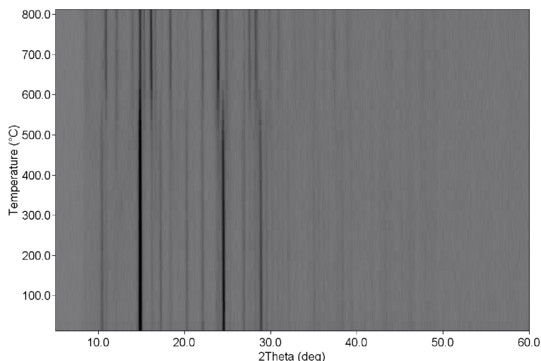
Fig. 7. High-temperature X-ray powder patterns of bixbyite-type V_2O_{3.07}N_{0.13} in argon atmosphere. Above \sim 550^\circ C a corundum-type phase ( V_2O_3 ) is observed.
