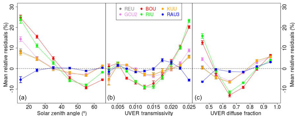
Figure 3. Mean relative residuals of each UVER diffuse fraction model vs. (a) solar zenith angle, (b) UVER transmissivity, and (c) predicted UVER diffuse fraction values. The range of the solar zenith angle (10–70°) has been divided into six equal bins while the ranges of the k_{\text{UVER}} (0, 0.025) and f_{\text{UVER}} (0,1) have been split into 10 bins. The mean value for each bin (central point) and the standard deviation of the mean are shown (error bars)
