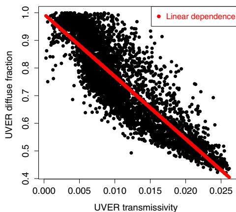
Figure 1. UVER diffuse fraction ( f_{\text{UVER}} ) vs. UVER transmissivity ( k_{\text{UVER}} ), and linear fitting.
