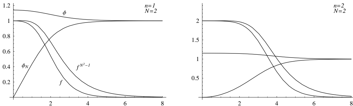
Figure 2: Profile functions for local vortices, for negative magnetic flux and \kappa_1/\kappa_2 = 1/2 .
