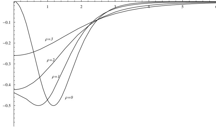
Figure 3: The magnetic field for semi-local vortices with \kappa_1 = \kappa_2 for different \rho values .
