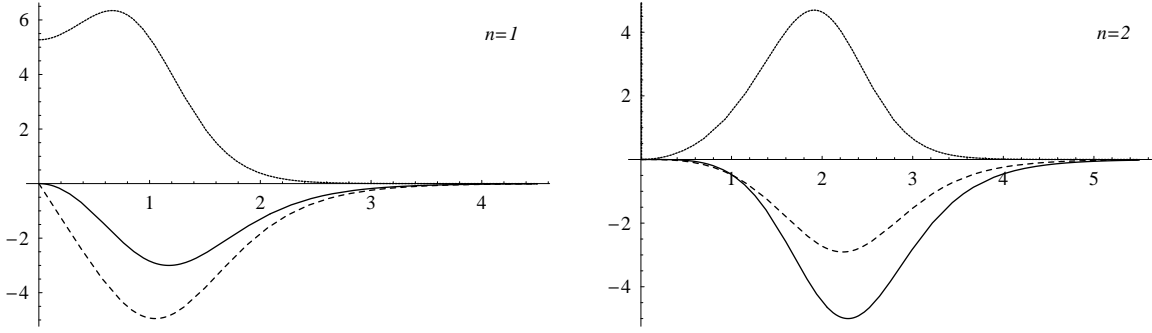
Figure 1: Plot of the magnetic field B^0 (solid line), electric field E^0 (dashed line), and energy density \mathcal{H} (dotted line) for local vortices with \kappa_1/\kappa_2 = 1 . The distance between the energy density maximum and the origin increases with the winding number n .
