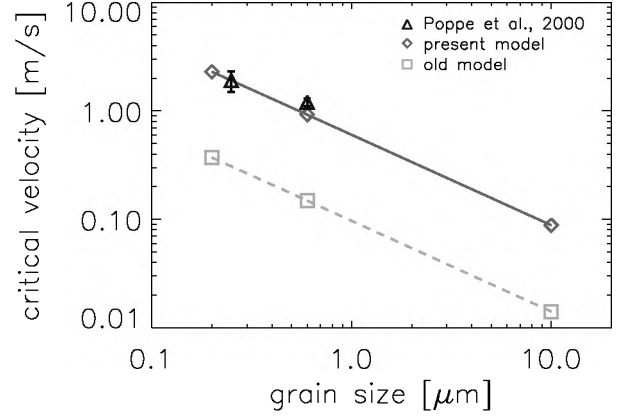
Fig. 1. Critical velocity as a function of a grain size. Squares indicate the model without additional dissipation process, diamonds show present model with the energy dissipation by plastic deformation of surface roughness and triangles show experimentally determined values by Poppe et al. (2000) with error bars.
