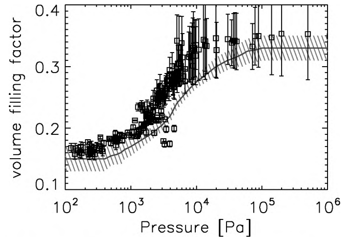
Fig. 5. The volume filling factor vs normal pressure. The solid line indicates the results of the laboratory experiment by Blum & Schr apler (2004). The dashed area is the error to that data. Squares show results of our single simulations. Error bars are due to difficulty in determination of the volume of the final aggregate.
