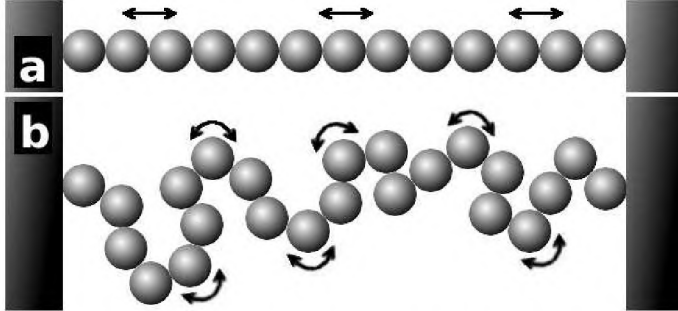
Fig. 6. Sketch of a sound wave propagation in a linear aggregate (a) and in a porous aggregate (b).
