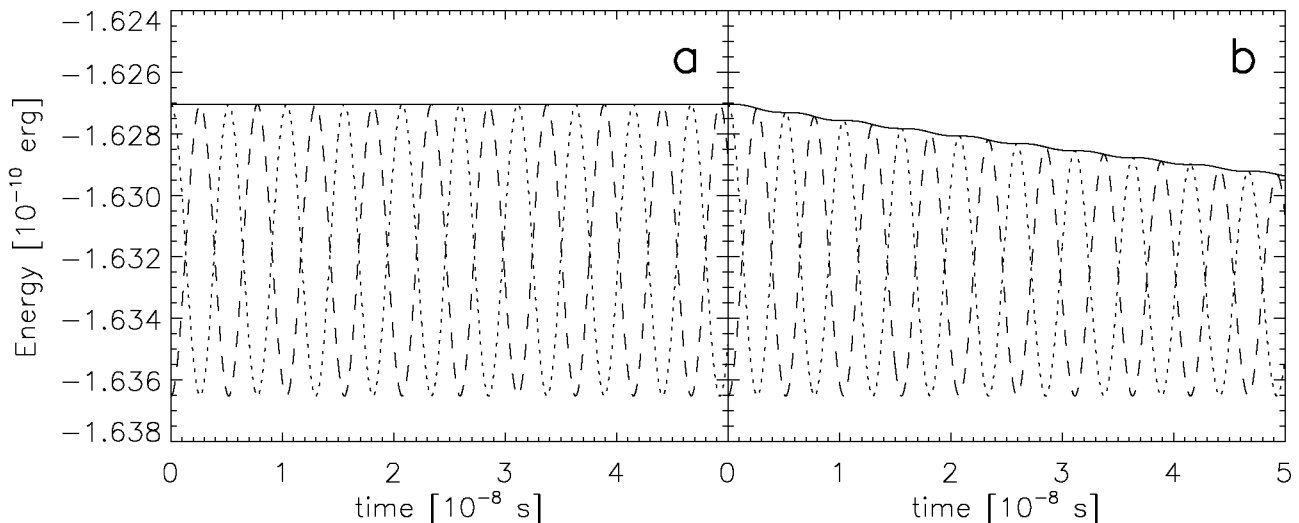
Fig. 2. The total energy is redistributed between the kinetic energy (dashed line) and the potential energy (dotted line). At the maximum and minimum separation the potential energy is maximum, while in the equilibrium position the kinetic energy is the highest. The kinetic energy was shifted down for better overview (see text). No damping case – a, and the energy leak form the system due to the damping force – b.
