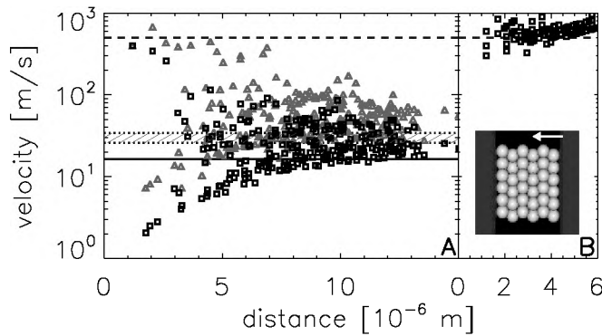
Fig. 7. Sound velocity in m/s versus distance from the plane that hits the aggregate. Squares indicate applied force of 5 \cdot 10^{-8} N and triangles 5 \cdot 10^{-6} N. The left panel (a) shows results of sound speed determination in a RBD aggregate, while the right one (b) in a CCP aggregate. The inset image shows the CCP aggregate placed in between two planes. The lines indicate sound velocities determined theoretically using vertical force in a linear chain of monomers (dashed line) and using rolling friction (solid line). The Dashed area limited by dotted lines indicates the sound speed range determined experimentally by Teiser (2007)
