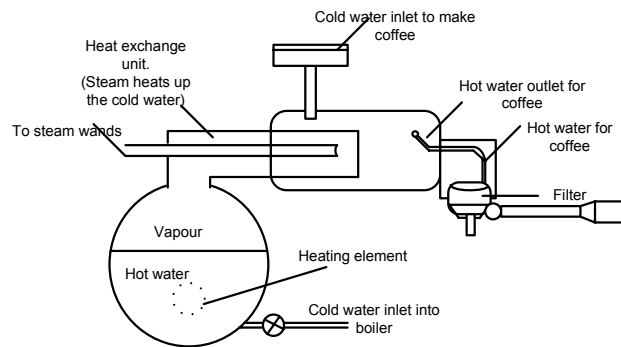
Fig. 1. The coffee machine blueprint.
