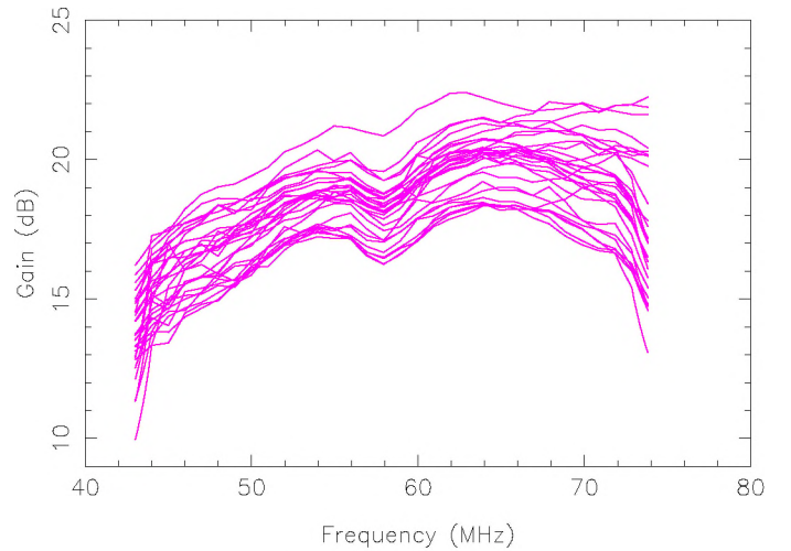
Figure 2. Electronics gain factors are plotted for all 30 LOPES antennae. The factors are for the correction of the received voltage measured in several calibration campaigns at KASCADE in the band from 43 MHz to 74 MHz.
