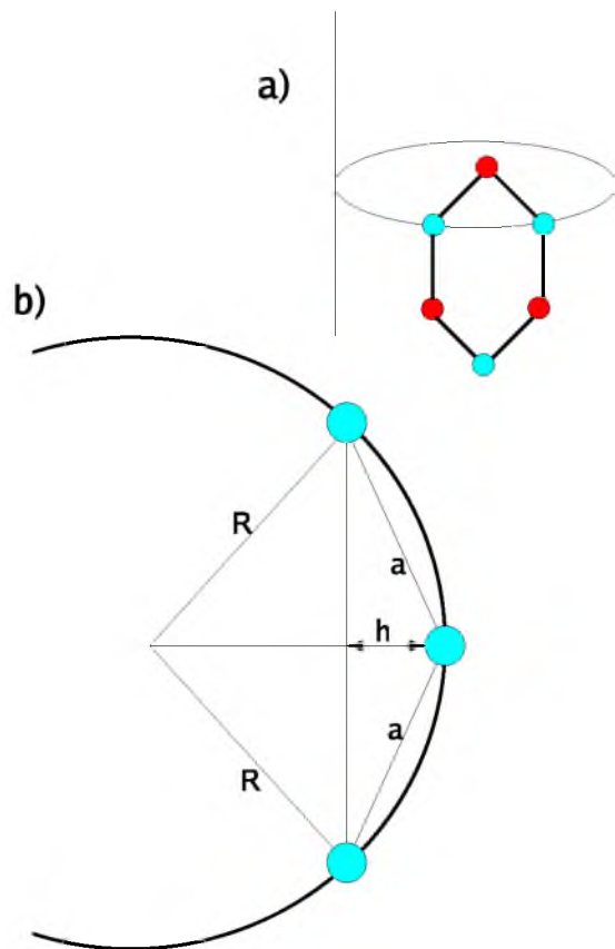
FIG. 8: (color online) (a) Position of carbon hexagons on surface of SWCNT. Red (dark) and blue (light) circles are carbon atoms from different sublattices. (b) Position of carbon atoms on radii of SWCNT.
