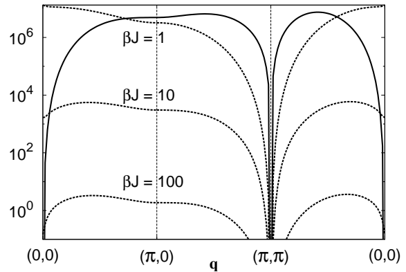
FIG. 6: Comparison between spectral weight for single-magnon scattering W_1 (dashed lines) for various temperatures and zero temperature two-magnon scattering W_2 (solid line), all obtained numerically. The figure displays the T^3 behavior from Eq. (32) for the single-magnon intensity. For \text{La}_2\text{CuO}_4 J \approx 146 meV, and at room temperature we have \beta_{\text{rt}}J \approx 5.8 .
