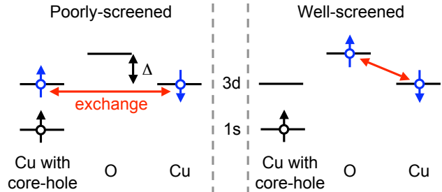
FIG. 2: Modification of the superexchange interaction in the well- and poorly-screened intermediate states. In the poorly-screened state, the core-hole potential U_c modifies the superexchange. For the well-screened state however, the copper 3d hole on the core-hole site is transferred to a neighboring oxygen, and superexchange is only of order \mathcal{O}(t_{pd}^2) , independent of U_c .
