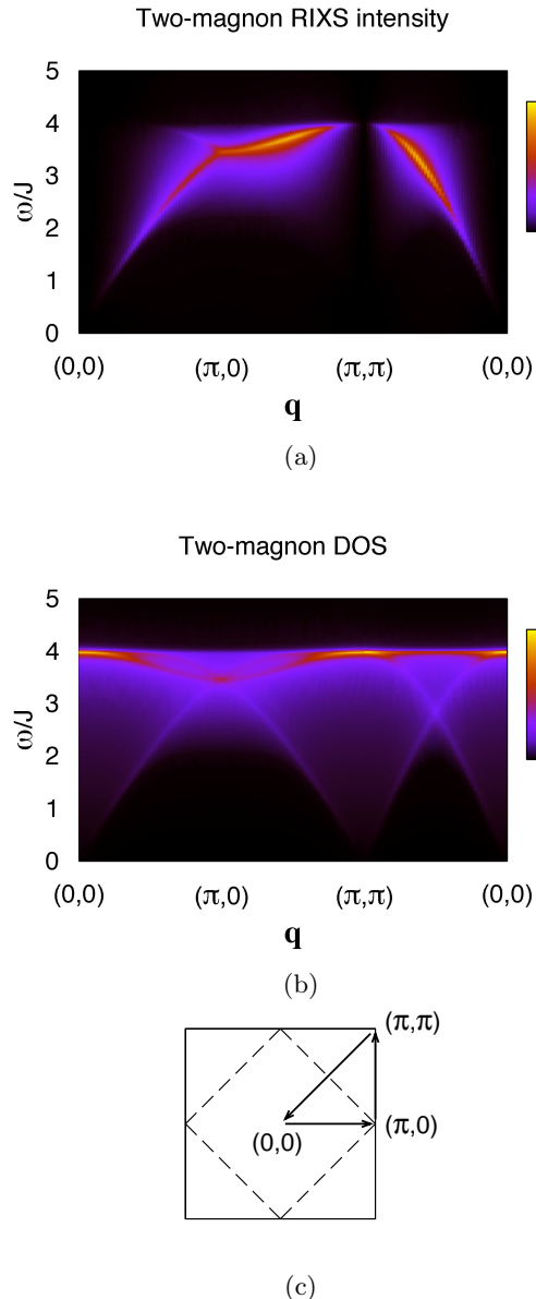
FIG. 3: RIXS spectrum (a) and two-magnon DOS (b) for a nearest neighbor Heisenberg antiferromagnet with exchange interaction J as a function of transferred momentum \mathbf{q} for a cut through the Brillouin zone (c). The dashed line indicates the magnetic BZ boundary.
