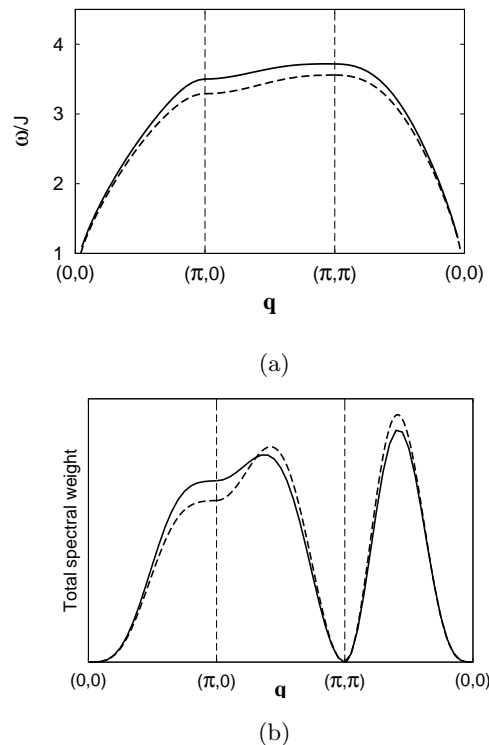
FIG. 4: First moment (a) and total spectral weight (b) of the RIXS spectrum. The solid lines are obtained by using interaction strengths determined from neutron data (next neighbor coupling J = 146.3 meV, second and third neighbor couplings J' = J'' = 2 meV and ring exchange J_c = 61 meV). 29 The dashed lines have only nearest neighbor interaction.
