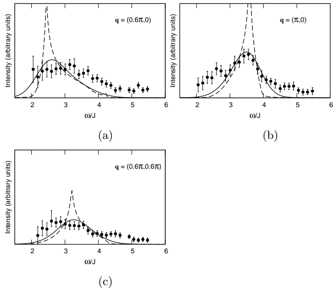
FIG. 5: RIXS intensity for various points in the BZ. Each figure contains the bare theoretical data (dashed line), the convolution with experimental resolution (solid line), and the experimental data from Ref. 17. For these figures, we used J = 146.3 meV, second and third neighbor couplings J' = J'' = 2 meV and ring exchange J_c = 61 meV. The latter contribution is evaluated theoretically using a mean field approximation. These values were found in neutron scattering experiments. 29 These experiments were analyzed using the wave-vector independent renormalization factor Z_c = 1.18 , which is also used to generate the theoretical curves. The theoretical intensity is scaled independently in each figure to match the experiment. The overall scale factors differ at most by a factor 2.5, which is comparable to experimental uncertainty in absolute intensities. 39
